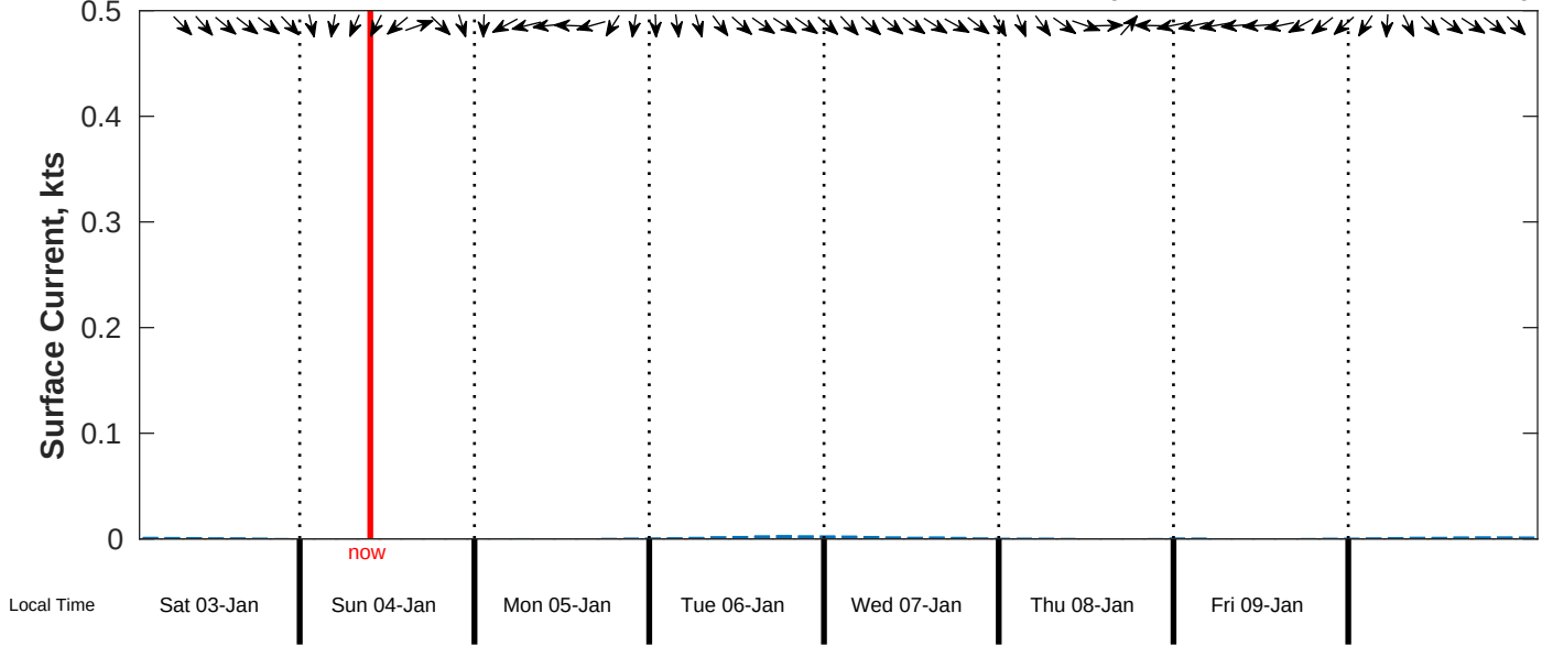
Surface Current Forecast for CSA (ONHYM) PPL EBS - Sierra Leone from 03-Jan-2026 00:00:00 to 11-Jan-2026 00:00:00
