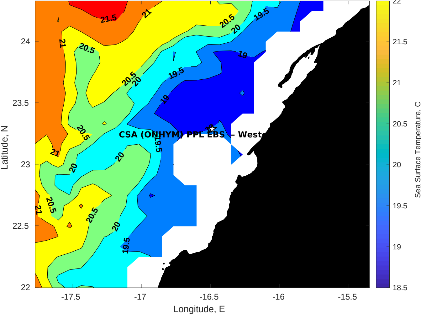
SST for CSA (ONHYM) PPL EBS - Western Sahara at 03-Jan-2026 00:00:00
