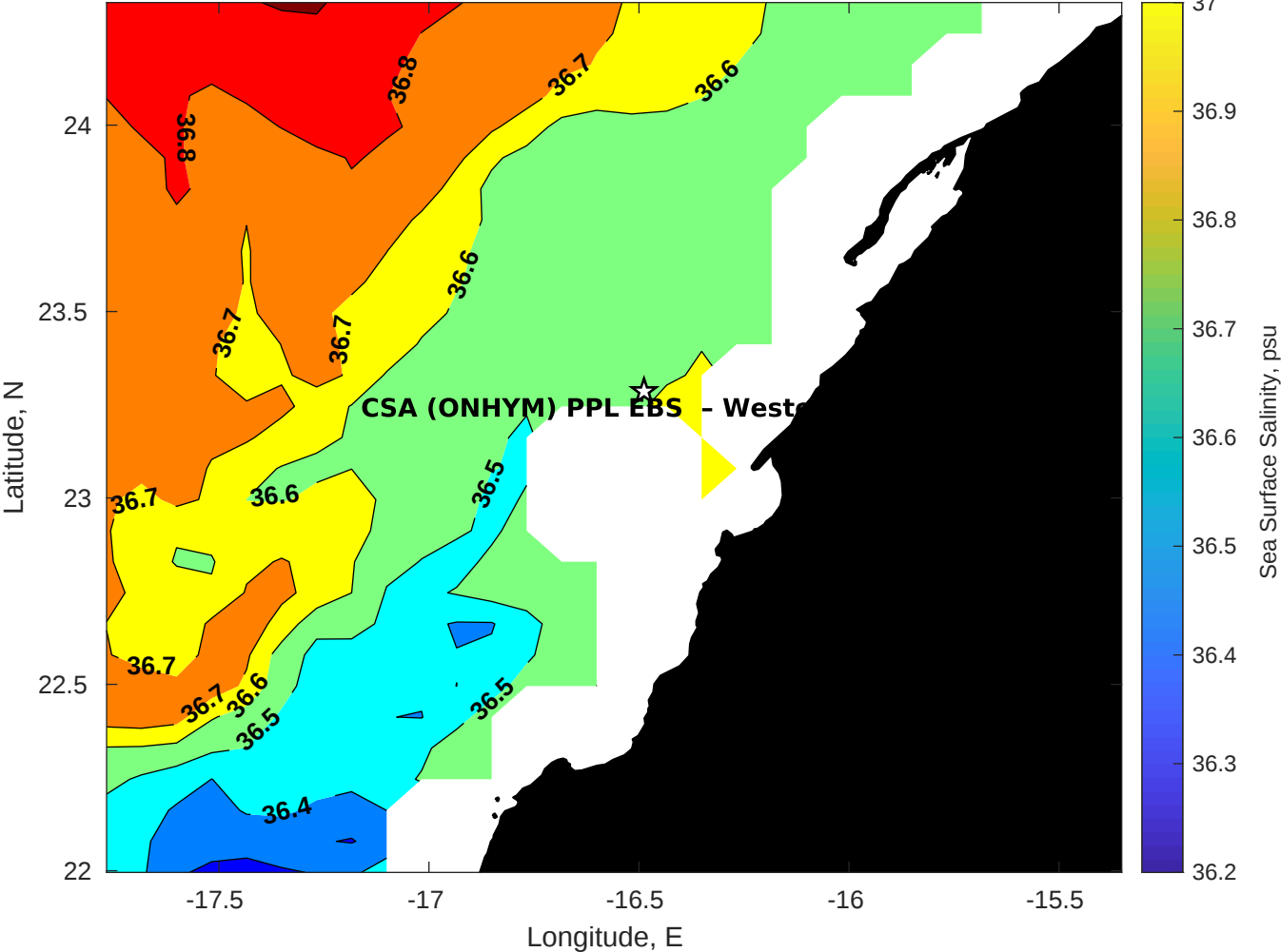
Surface Salinity for CSA (ONHYM) PPL EBS - Western Sahara at 03-Jan-2026 00:00:00
