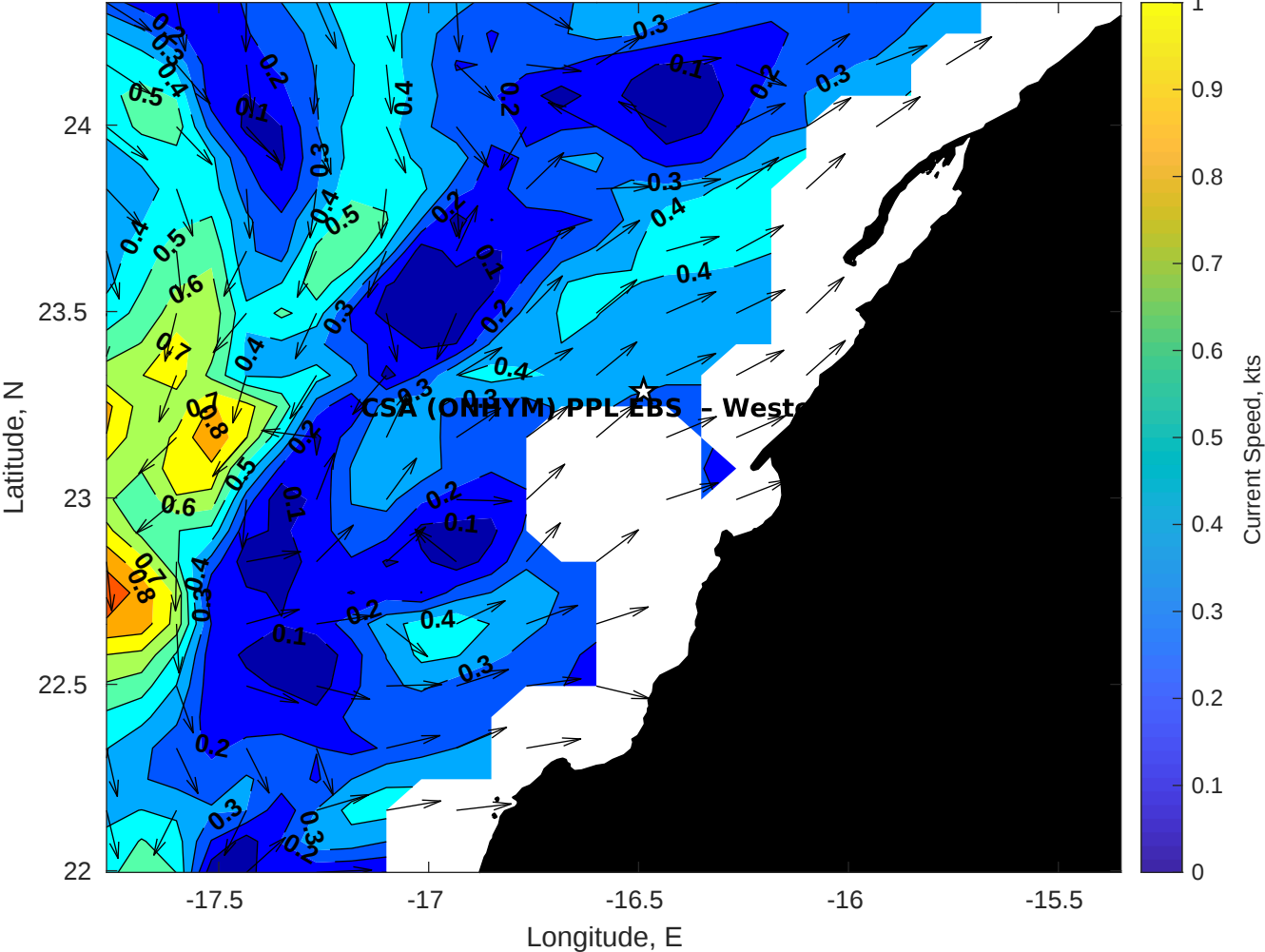
Surface Currents for CSA (ONHYM) PPL EBS - Western Sahara at 03-Jan-2026 00:00:00
