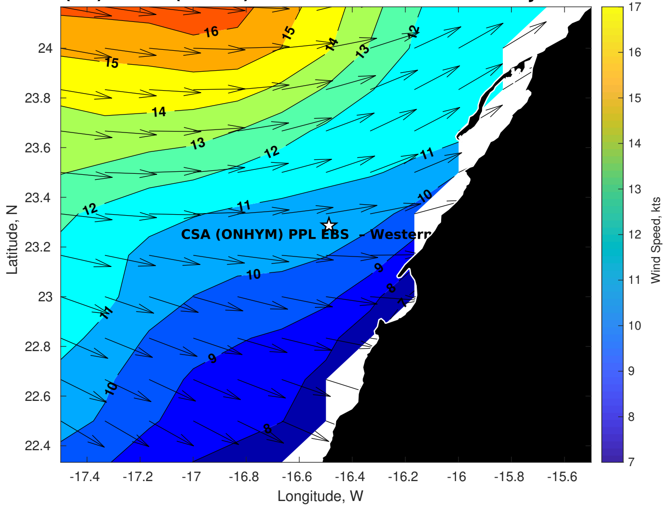
GFS Winds (kts) for CSA (ONHYM) PPL EBS - Western Sahara at 04-Jan-2026 09:00:00
