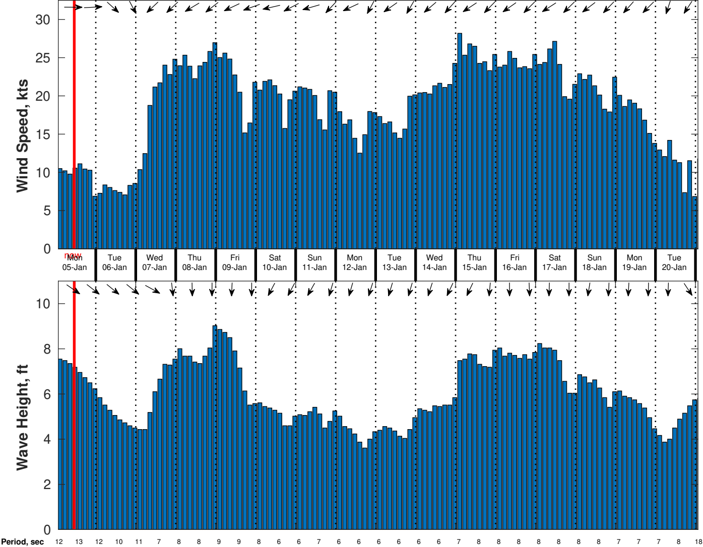
Wind & Wave Forecast for CSA (ONHYM) PPL EBS - Western Sahara from 04-Jan-2026 01:00:00 to 20-Jan-2026 01:00:00
