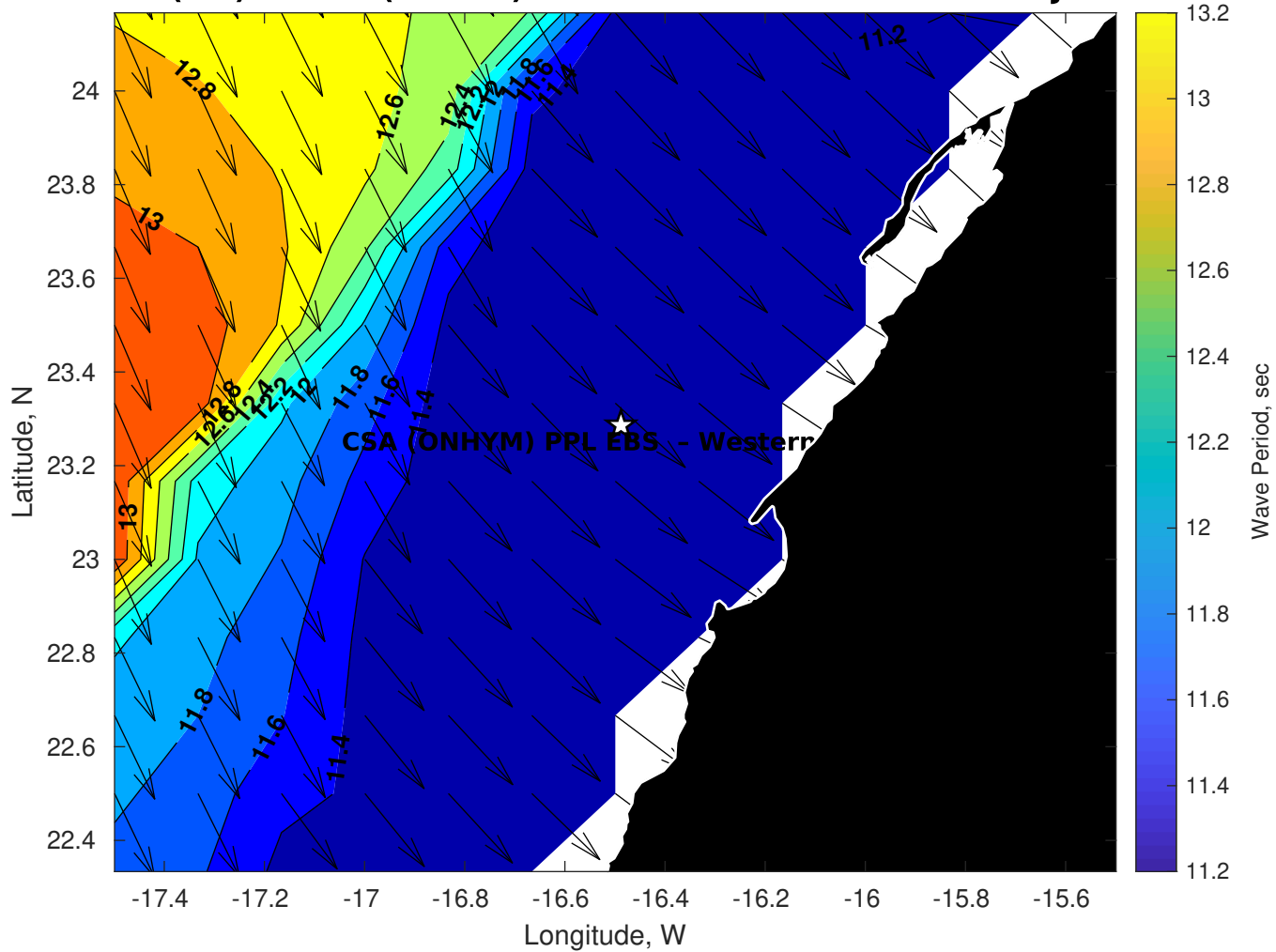
GFS Wave Period (sec) for CSA (ONHYM) PPL EBS - Western Sahara at 04-Jan-2026 09:00:00
