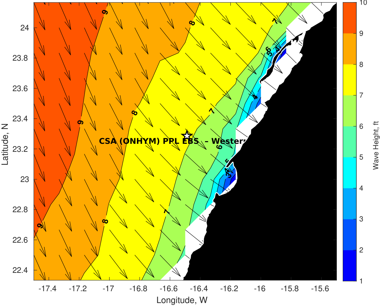
GFS Wave Height (ft) for CSA (ONHYM) PPL EBS - Western Sahara at 04-Jan-2026 09:00:00
