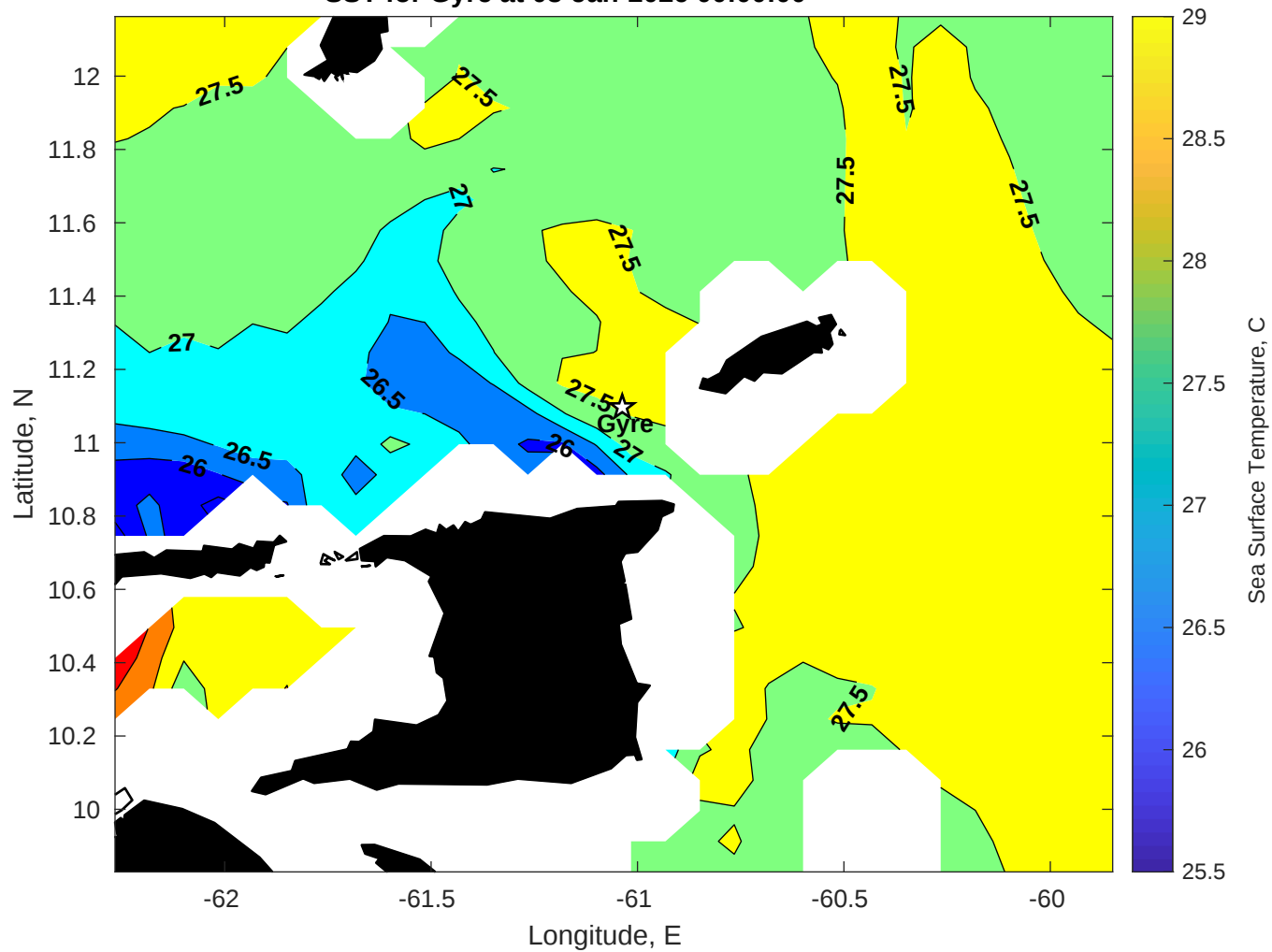
SST for Gyre at 03-Jan-2026 00:00:00
