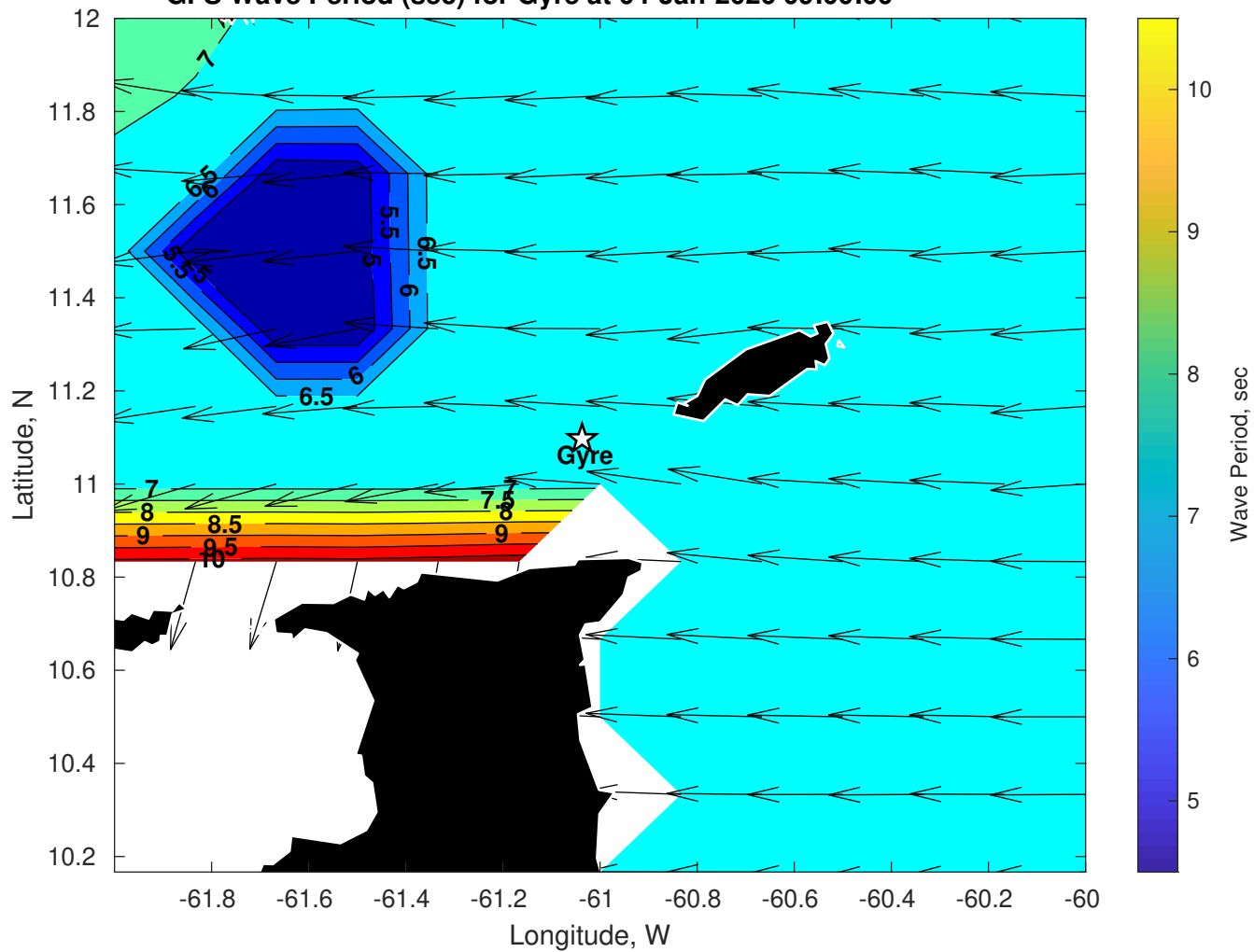
GFS Wave Period (sec) for Gyre at 04-Jan-2026 09:00:00
