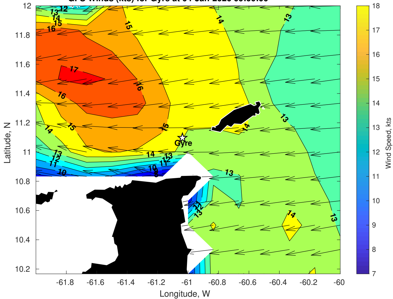
GFS Winds (kts) for Gyre at 04-Jan-2026 09:00:00
