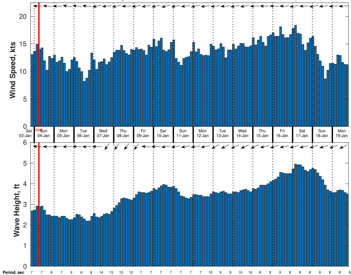
Wind & Wave Forecast for Gyre from 03-Jan-2026 20:00:00 to 19-Jan-2026 20:00:00
