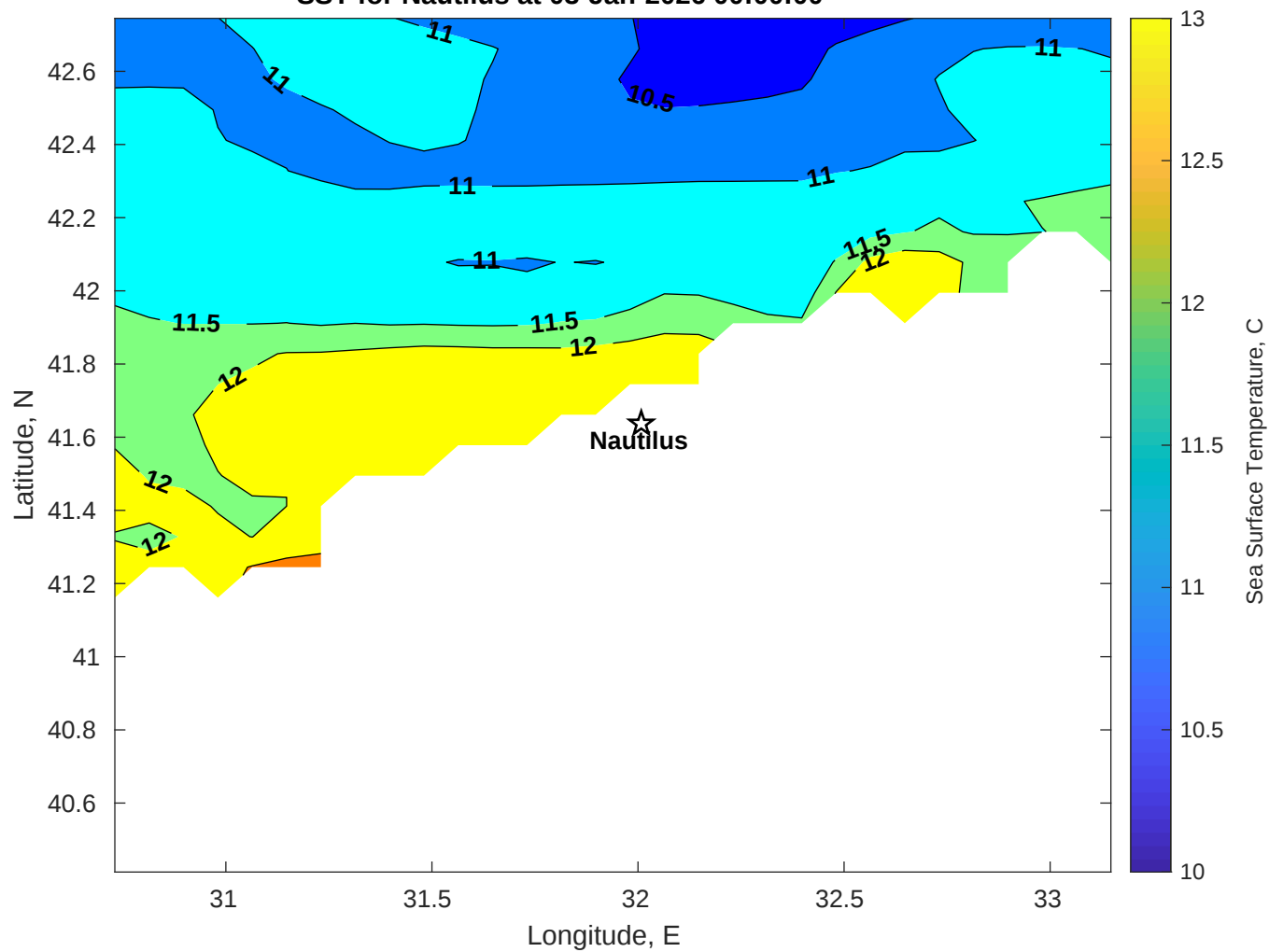
SST for Nautilus at 03-Jan-2026 00:00:00
