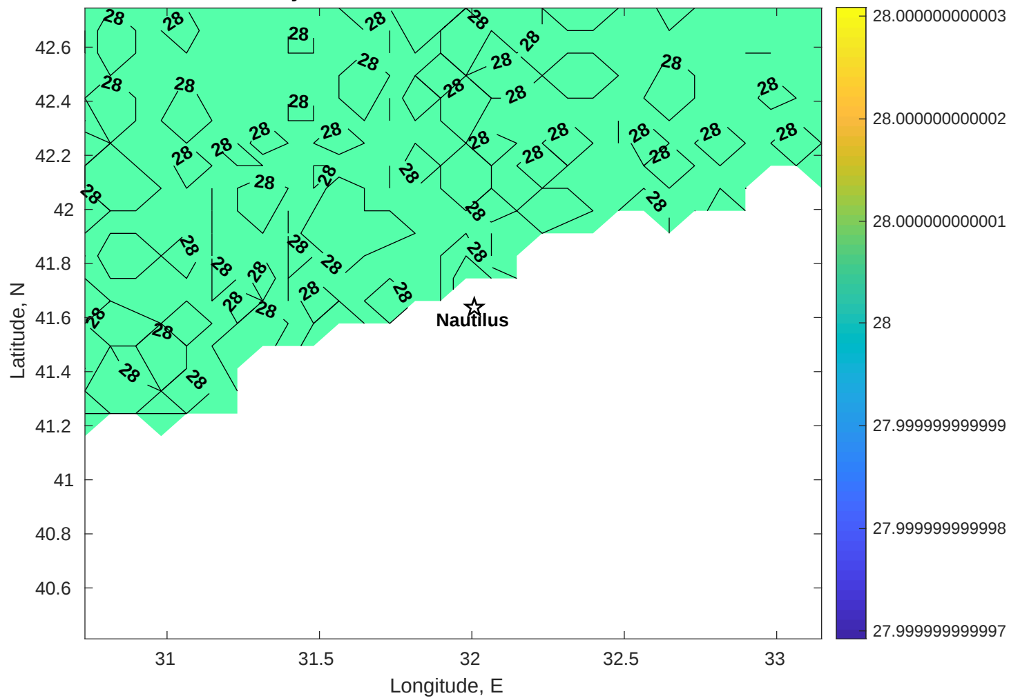
Surface Salinity for Nautilus at 03-Jan-2026 00:00:00
