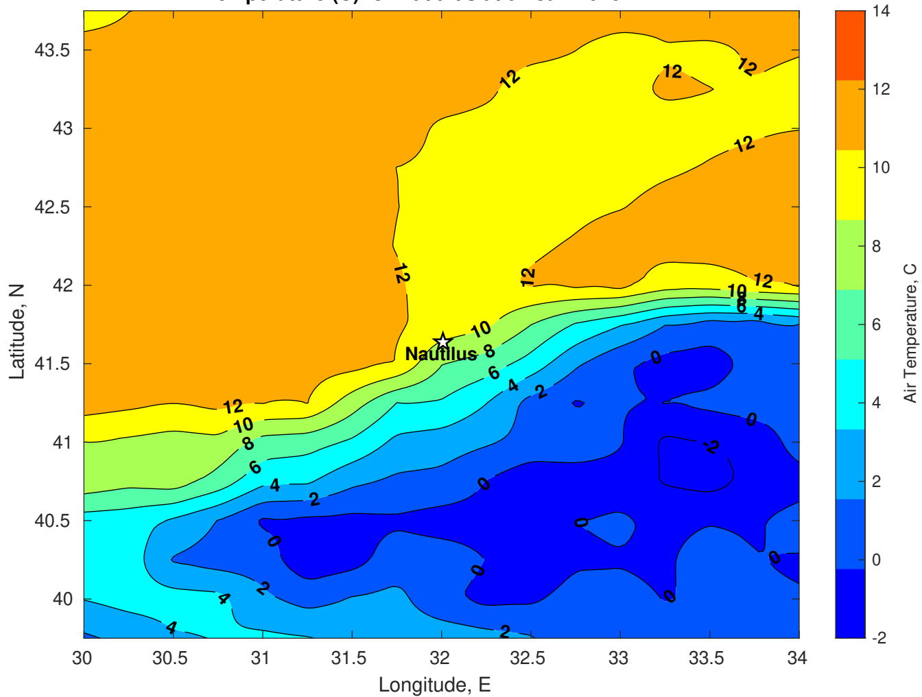
Air Temperature (C) for Nautilus at 04-Jan-2026
