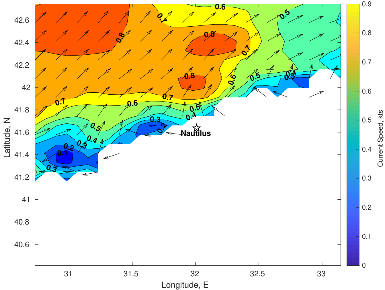
Surface Currents for Nautilus at 03-Jan-2026 00:00:00
