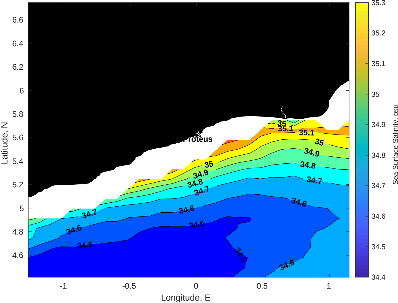
Surface Salinity for Proteus at 03-Jan-2026 00:00:00
