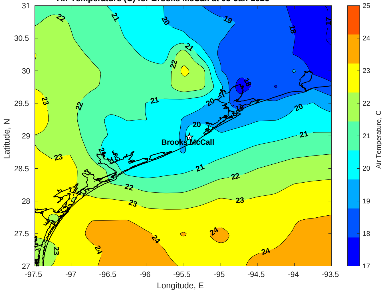
Air Temperature (C) for Brooks McCall at 05-Jan-2026
