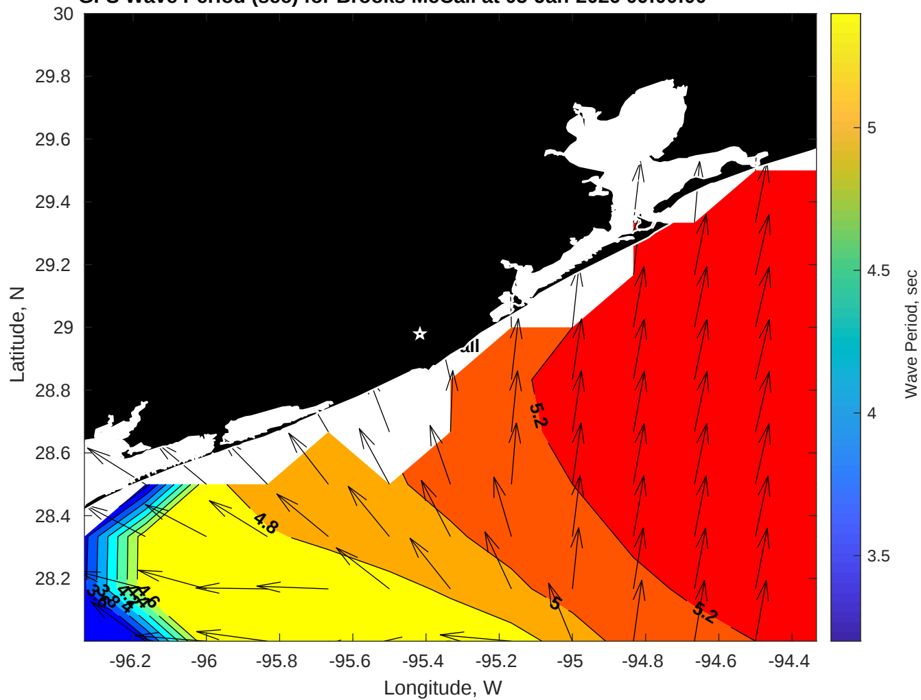
GFS Wave Period (sec) for Brooks McCall at 05-Jan-2026 09:00:00
