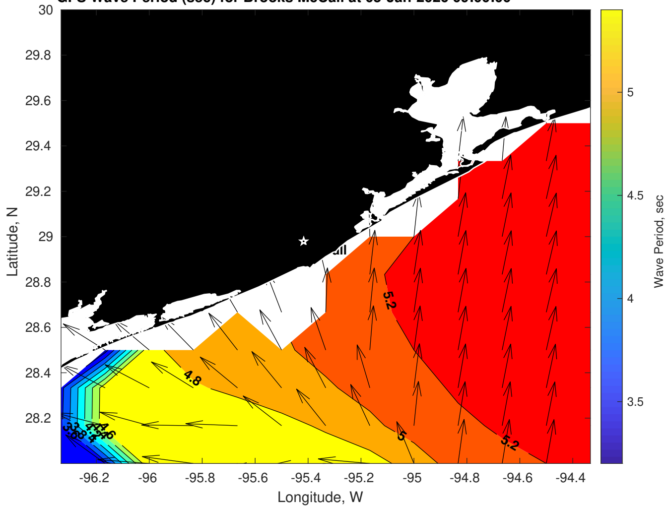
GFS Wave Period (sec) for Brooks McCall at 05-Jan-2026 09:00:00
