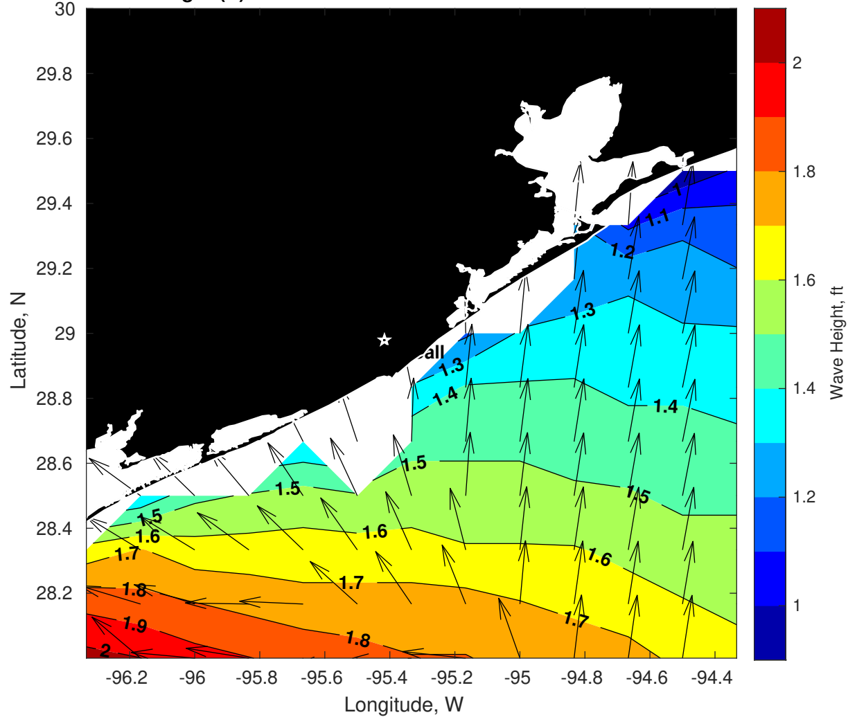
GFS Wave Height (ft) for Brooks McCall at 05-Jan-2026 09:00:00
