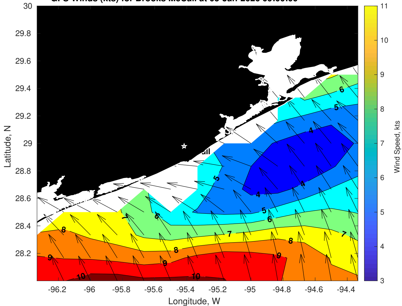
GFS Winds (kts) for Brooks McCall at 05-Jan-2026 09:00:00
