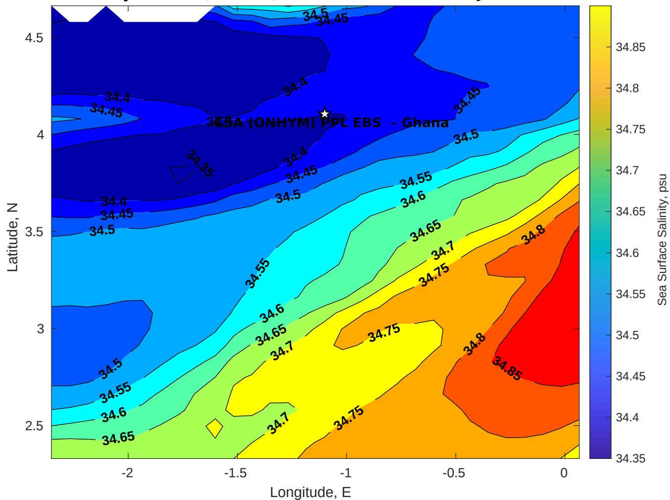
Surface Salinity for CSA (ONHYM) PPL EBS - Ghana at 04-Jan-2026 00:00:00
