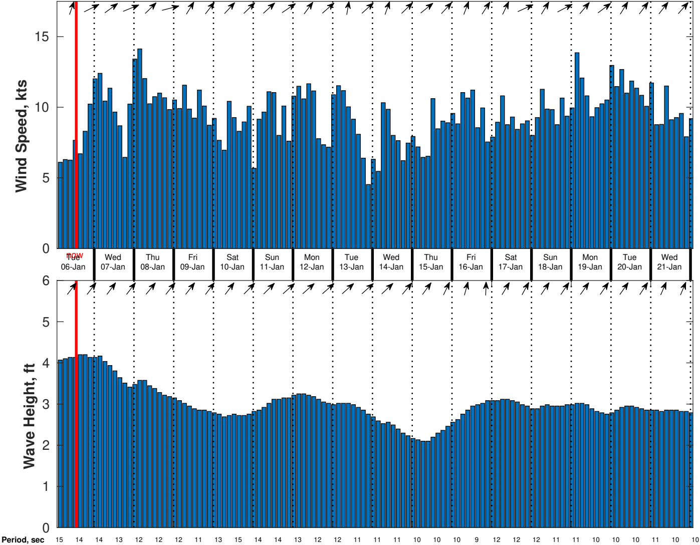
Wind & Wave Forecast for CSA (ONHYM) PPL EBS - Ghana from 05-Jan-2026 02:00:00 to 21-Jan-2026 02:00:00
