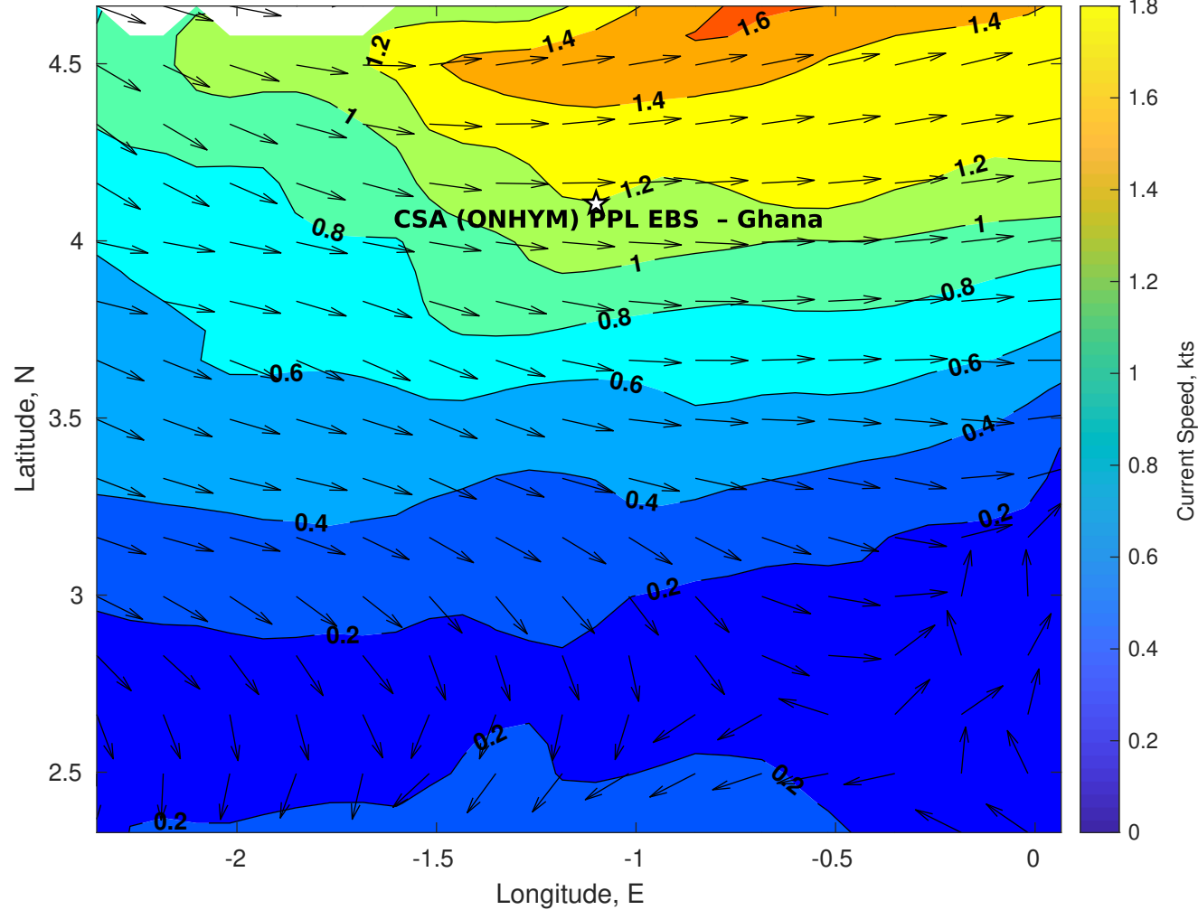
Surface Currents for CSA (ONHYM) PPL EBS - Ghana at 04-Jan-2026 00:00:00
