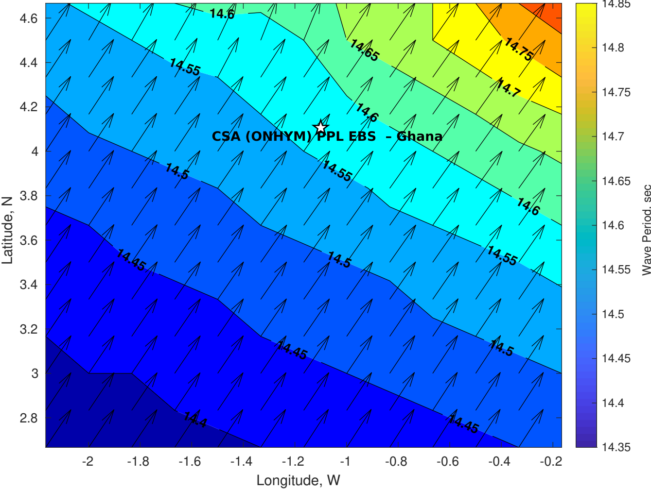
GFS Wave Period (sec) for CSA (ONHYM) PPL EBS - Ghana at 05-Jan-2026 09:00:00
