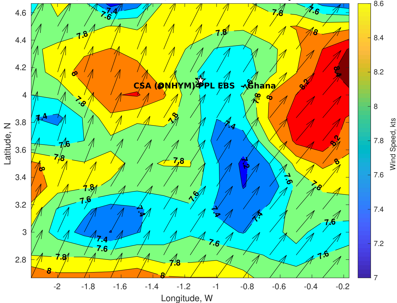
GFS Winds (kts) for CSA (ONHYM) PPL EBS - Ghana at 05-Jan-2026 09:00:00
