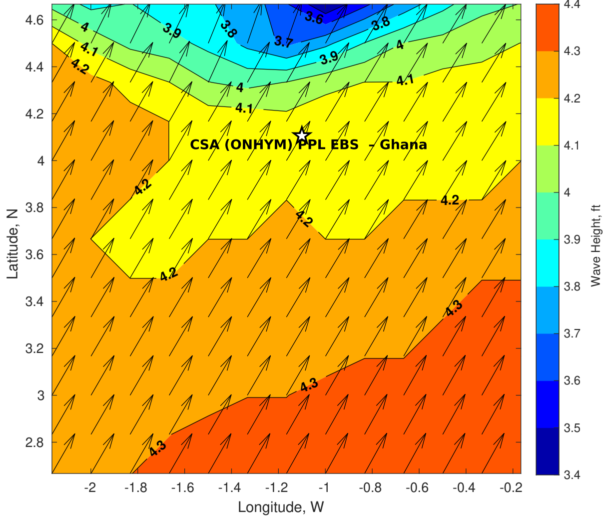
GFS Wave Height (ft) for CSA (ONHYM) PPL EBS - Ghana at 05-Jan-2026 09:00:00
