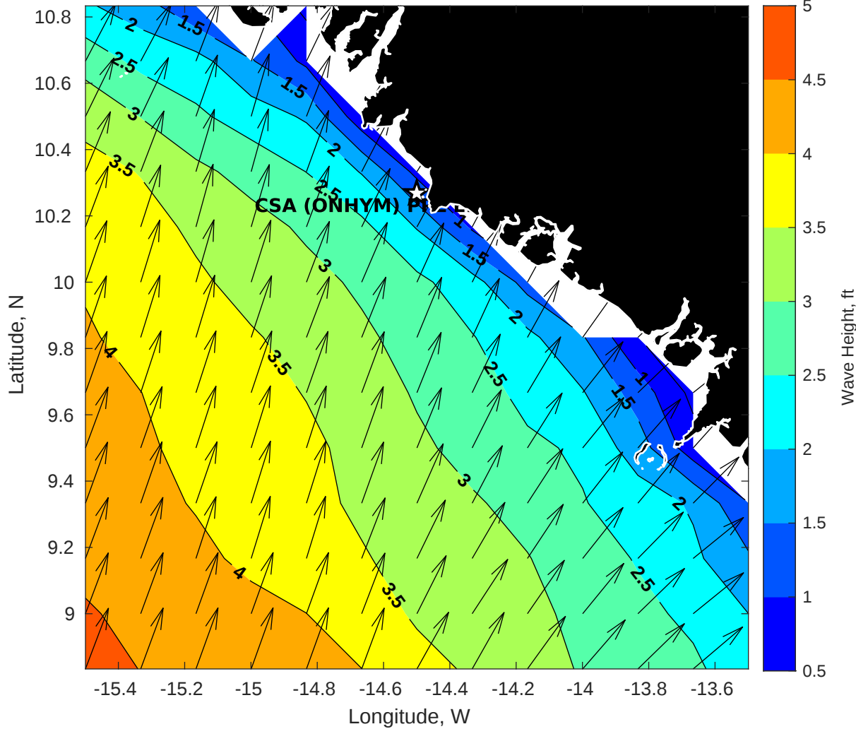
GFS Wave Height (ft) for CSA (ONHYM) PPL EBS - Guinea at 05-Jan-2026 09:00:00
