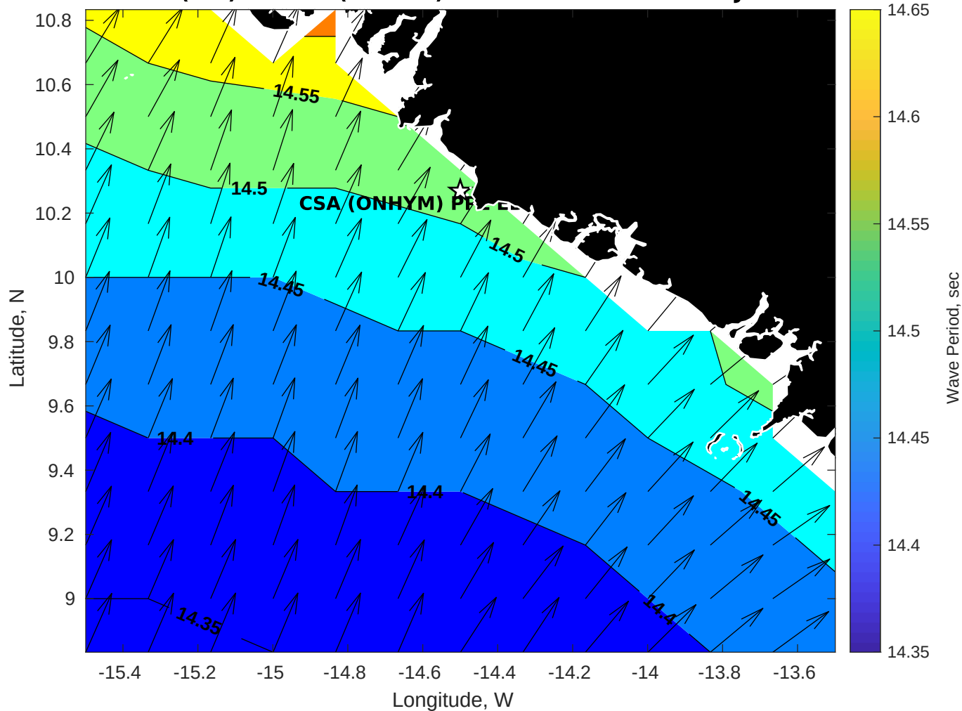
GFS Wave Period (sec) for CSA (ONHYM) PPL EBS - Guinea at 05-Jan-2026 09:00:00
