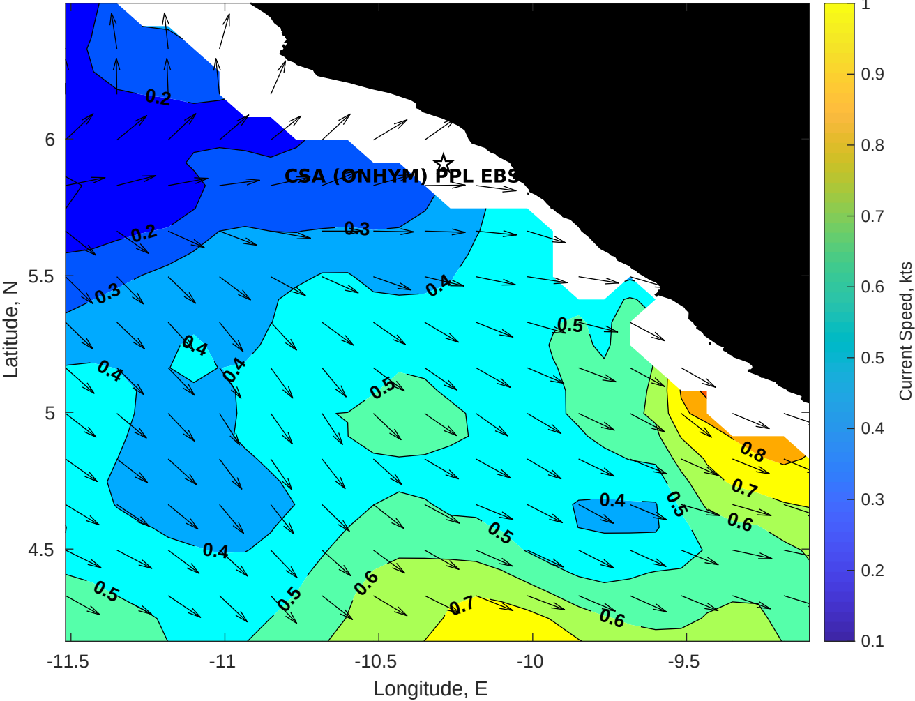
Surface Currents for CSA (ONHYM) PPL EBS - Liberia at 04-Jan-2026 00:00:00
