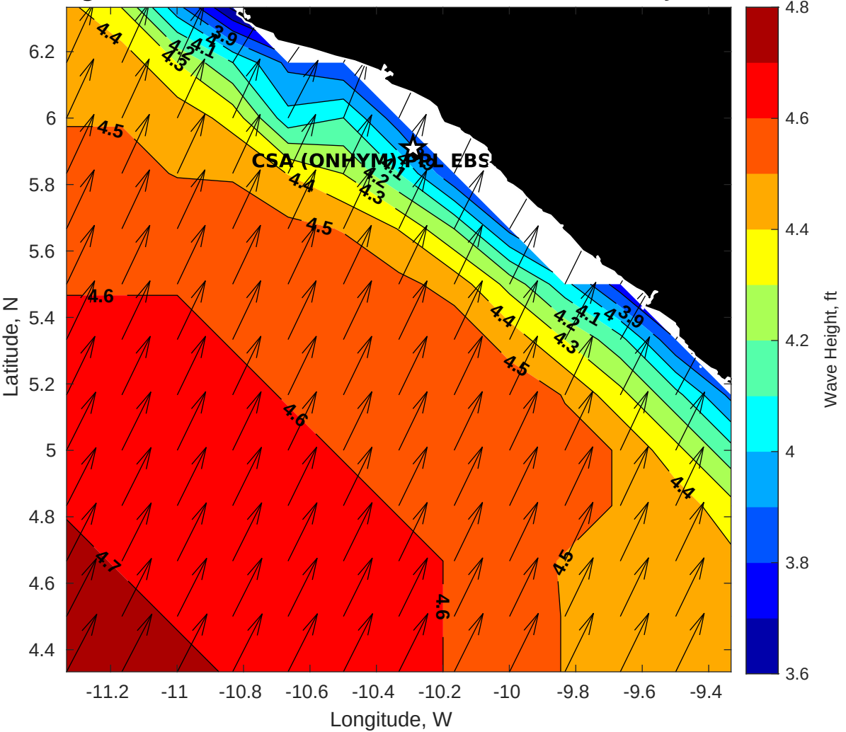
GFS Wave Height (ft) for CSA (ONHYM) PPL EBS - Liberia at 05-Jan-2026 09:00:00
