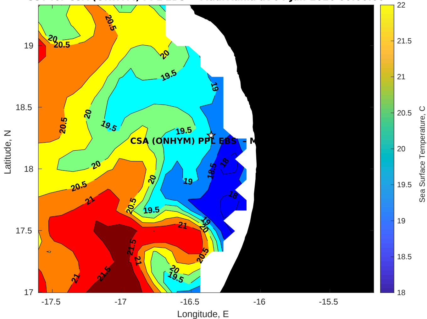
SST for CSA (ONHYM) PPL EBS - Mauritania at 04-Jan-2026 00:00:00
