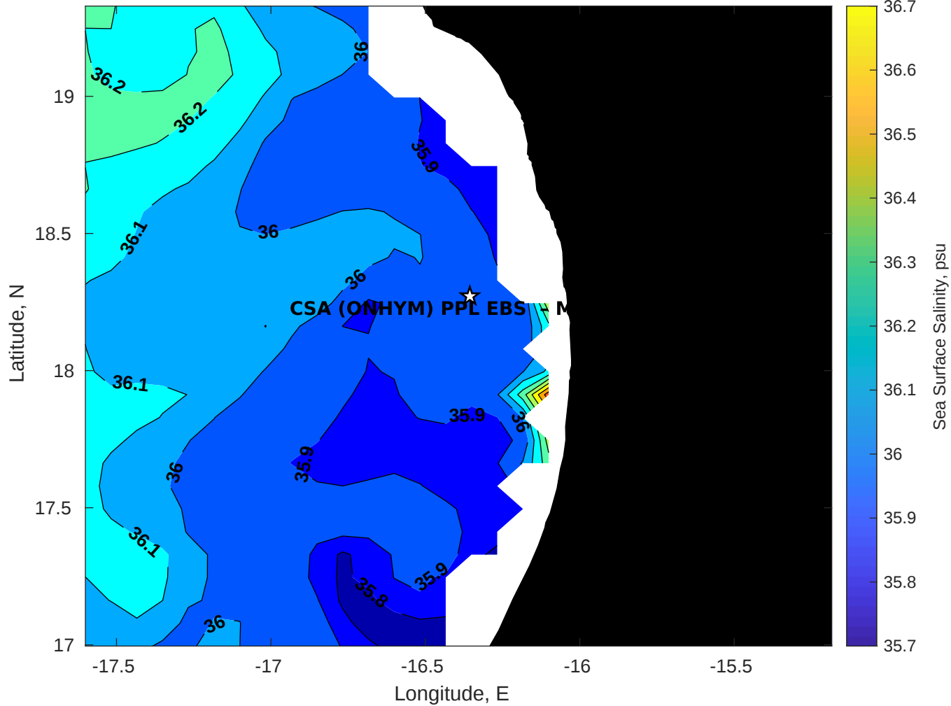
Surface Salinity for CSA (ONHYM) PPL EBS - Mauritania at 04-Jan-2026 00:00:00
