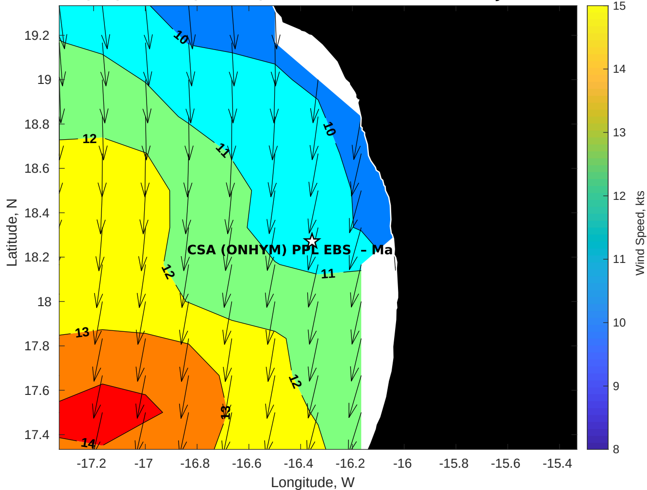
GFS Winds (kts) for CSA (ONHYM) PPL EBS - Mauritania at 05-Jan-2026 09:00:00
