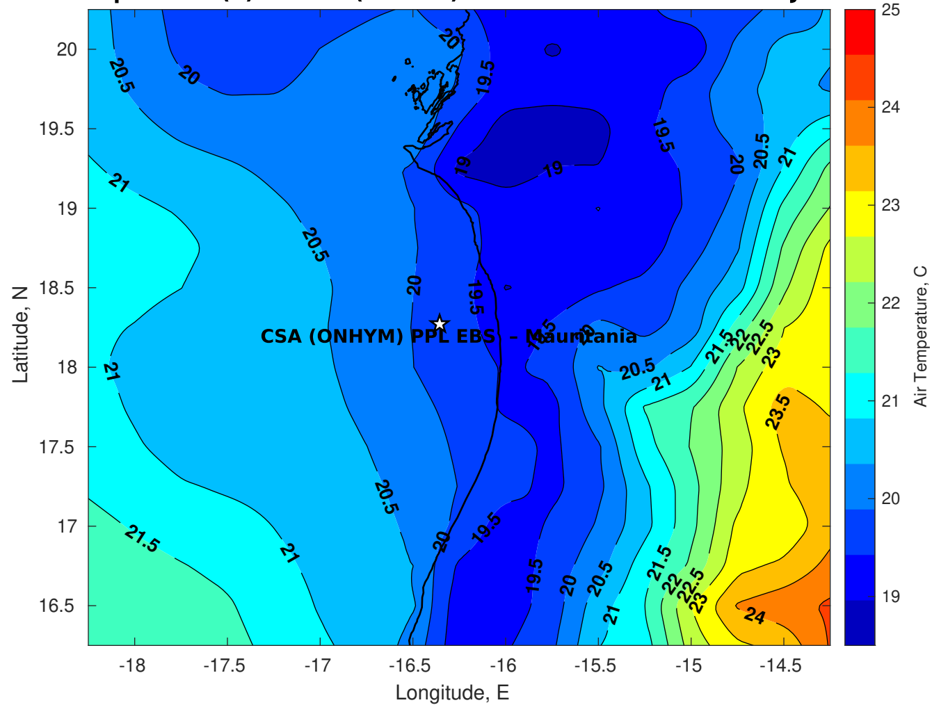
Air Temperature (C) for CSA (ONHYM) PPL EBS - Mauritania at 05-Jan-2026
