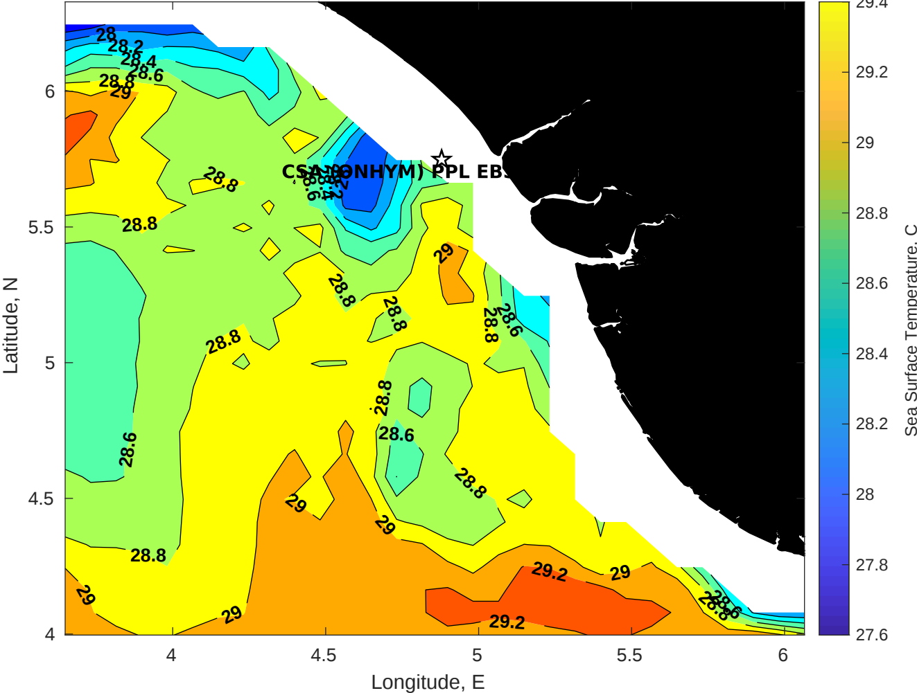
SST for CSA (ONHYM) PPL EBS - Nigeria at 04-Jan-2026 00:00:00
