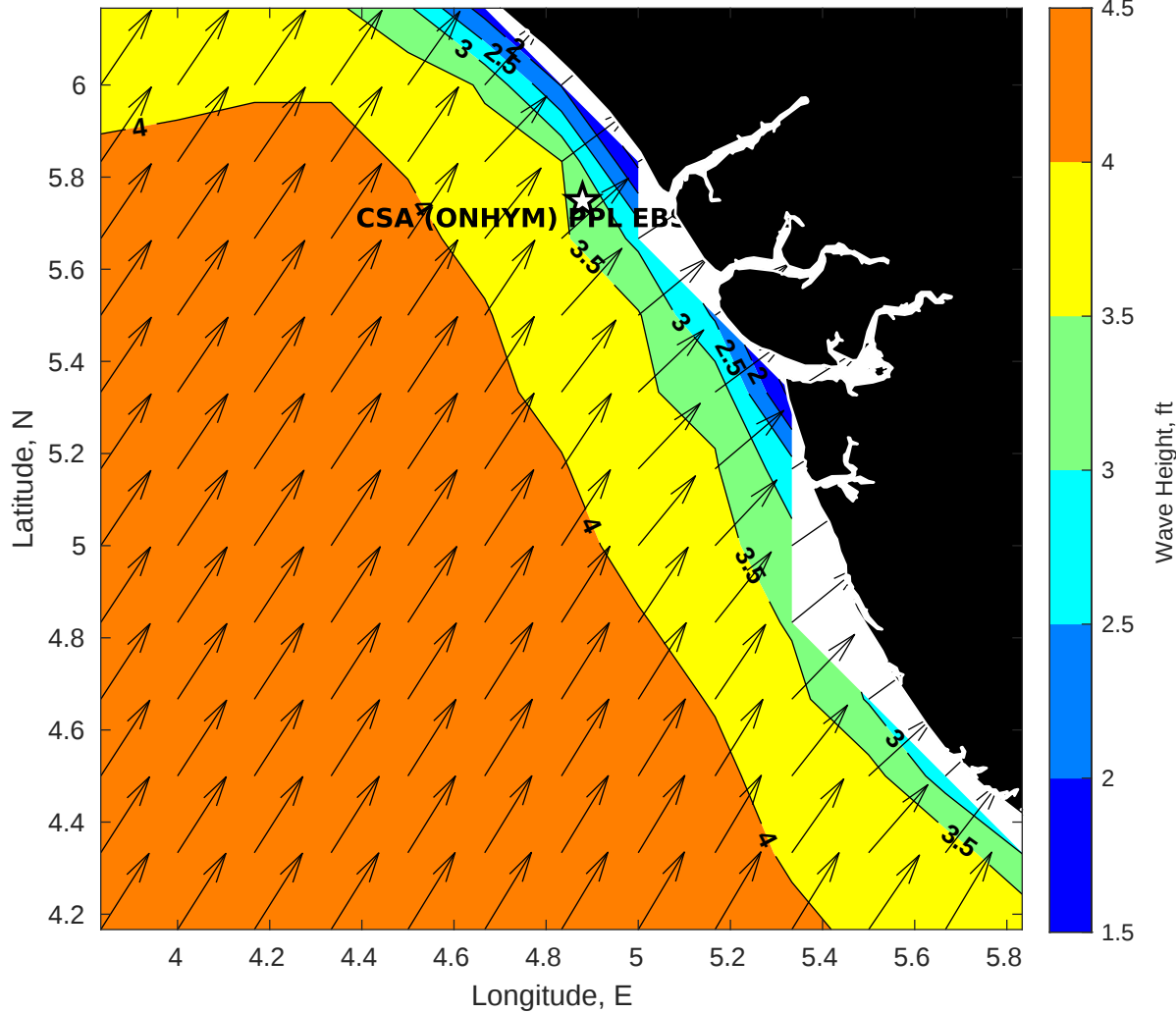
GFS Wave Height (ft) for CSA (ONHYM) PPL EBS - Nigeria at 05-Jan-2026 09:00:00
