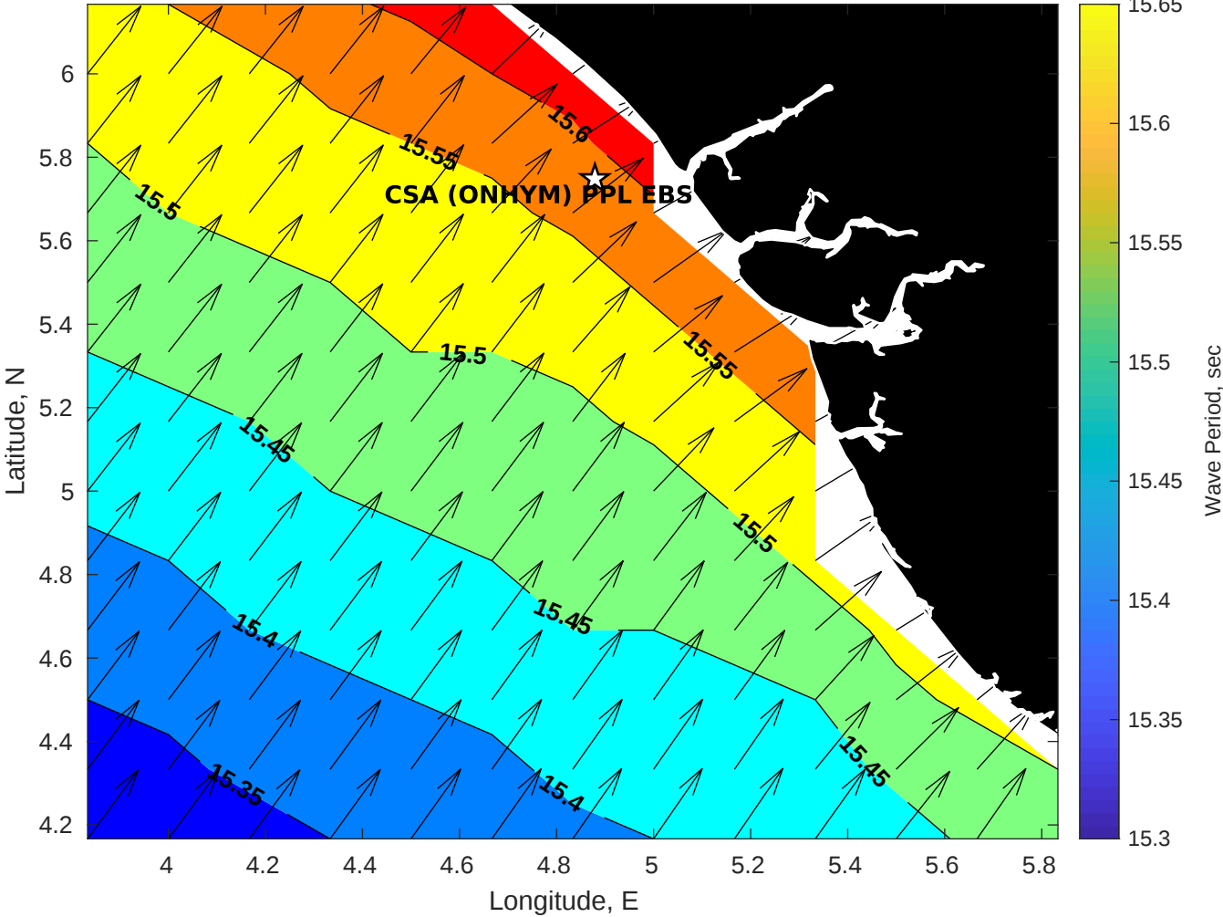
GFS Wave Period (sec) for CSA (ONHYM) PPL EBS - Nigeria at 05-Jan-2026 09:00:00
