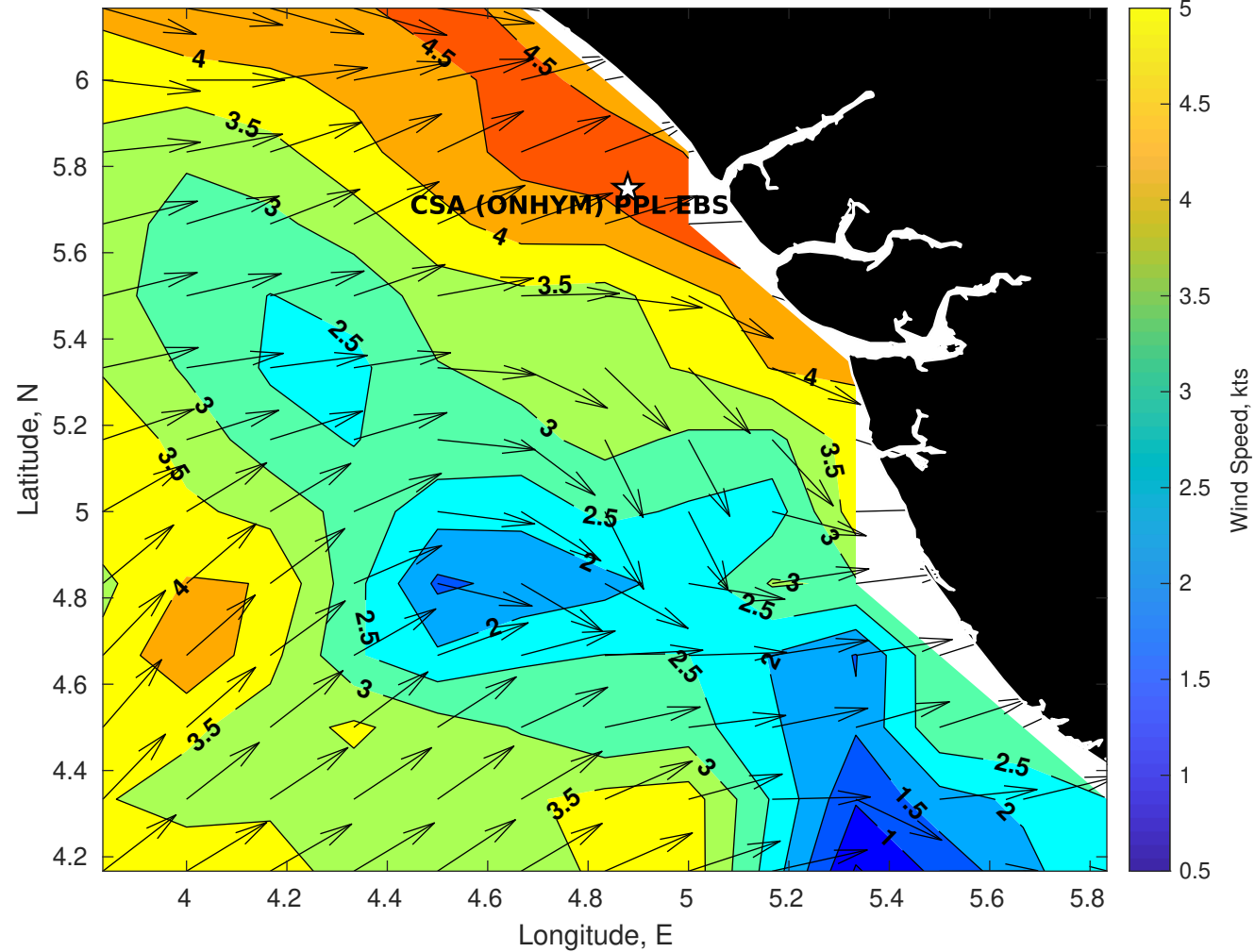
GFS Winds (kts) for CSA (ONHYM) PPL EBS - Nigeria at 05-Jan-2026 09:00:00
