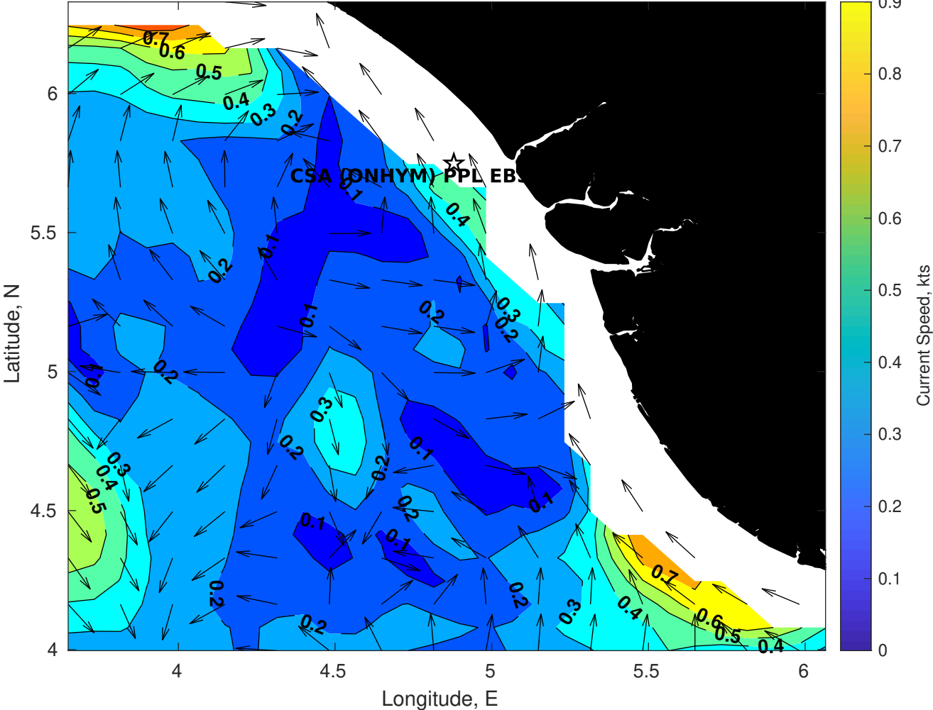
Surface Currents for CSA (ONHYM) PPL EBS - Nigeria at 04-Jan-2026 00:00:00
