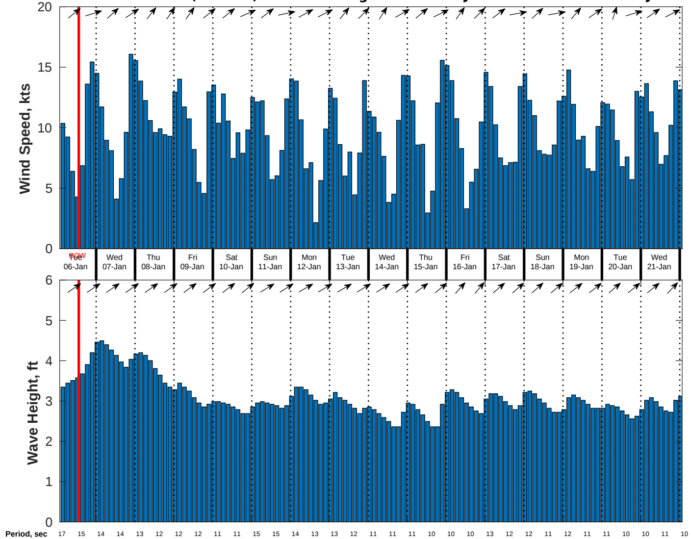
Wind & Wave Forecast for CSA (ONHYM) PPL EBS - Nigeria from 05-Jan-2026 02:00:00 to 21-Jan-2026 02:00:00
