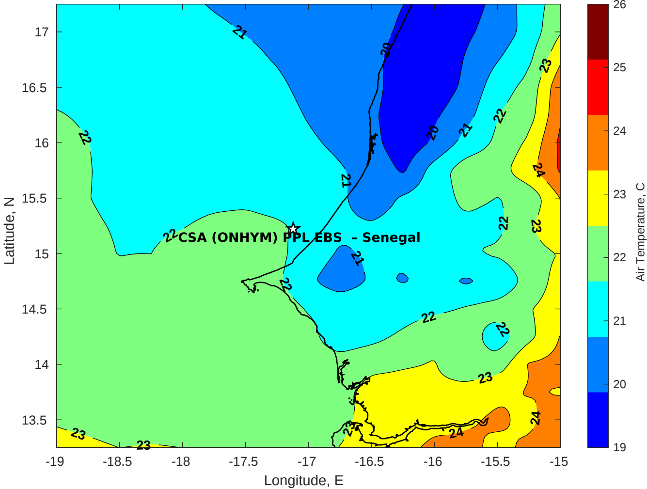
Air Temperature (C) for CSA (ONHYM) PPL EBS - Senegal at 05-Jan-2026
