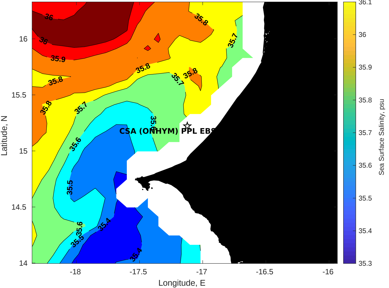
Surface Salinity for CSA (ONHYM) PPL EBS - Senegal at 04-Jan-2026 00:00:00
