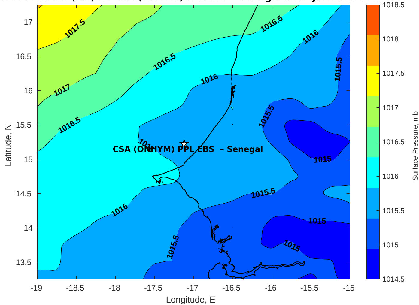
Surface Pressure (mb) for CSA (ONHYM) PPL EBS - Senegal at 07-Jan-2026 00:00:00
