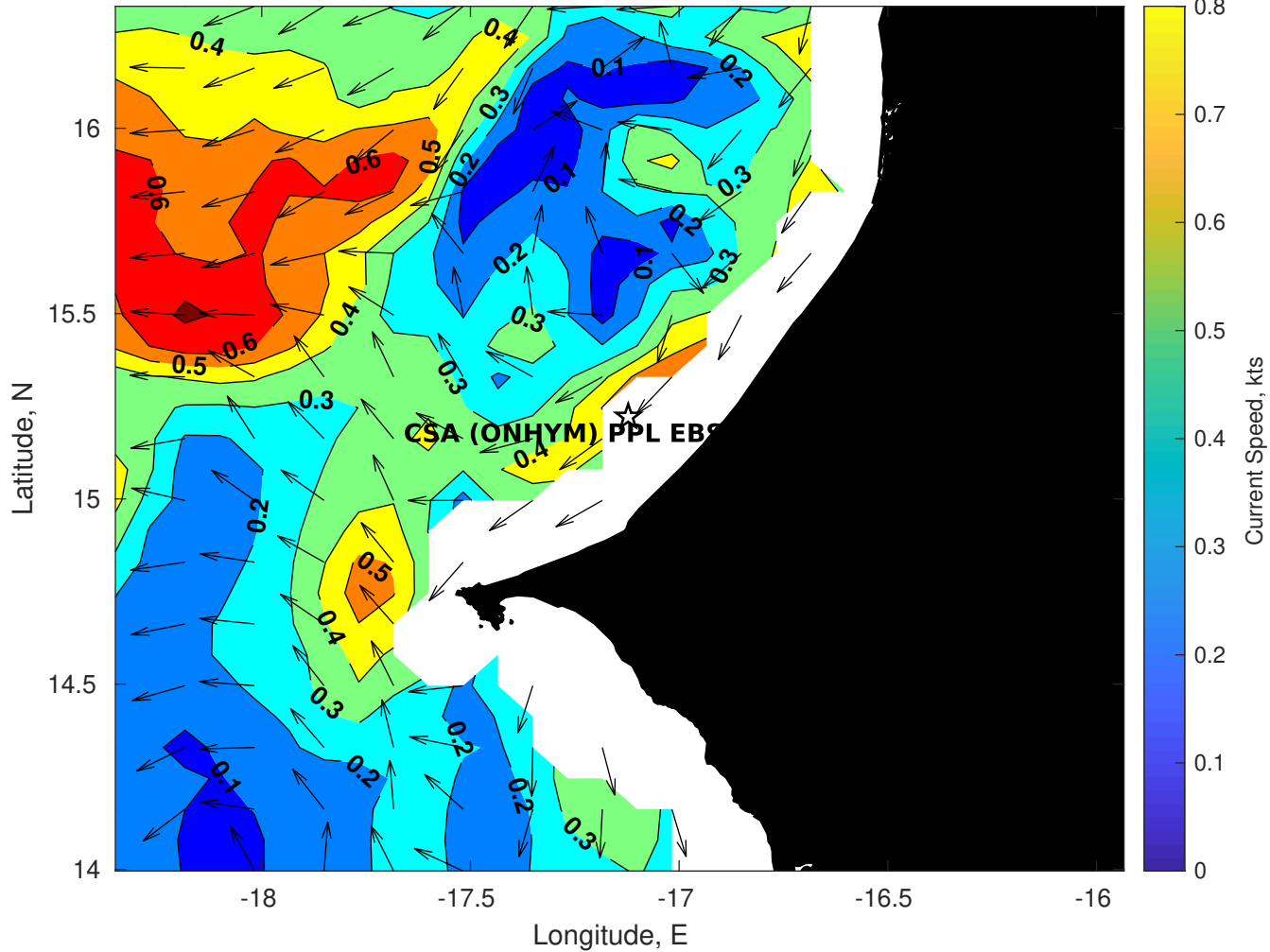
Surface Currents for CSA (ONHYM) PPL EBS - Senegal at 04-Jan-2026 00:00:00
