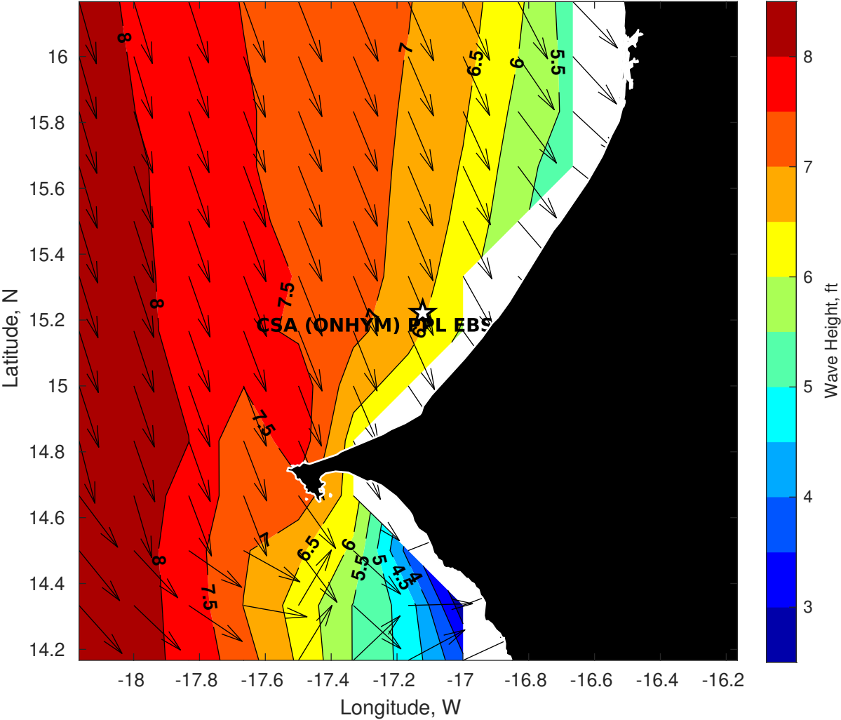
GFS Wave Height (ft) for CSA (ONHYM) PPL EBS - Senegal at 05-Jan-2026 09:00:00
