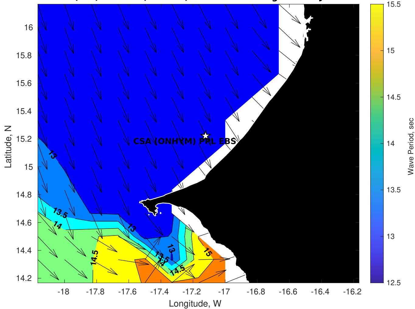
GFS Wave Period (sec) for CSA (ONHYM) PPL EBS - Senegal at 05-Jan-2026 09:00:00
