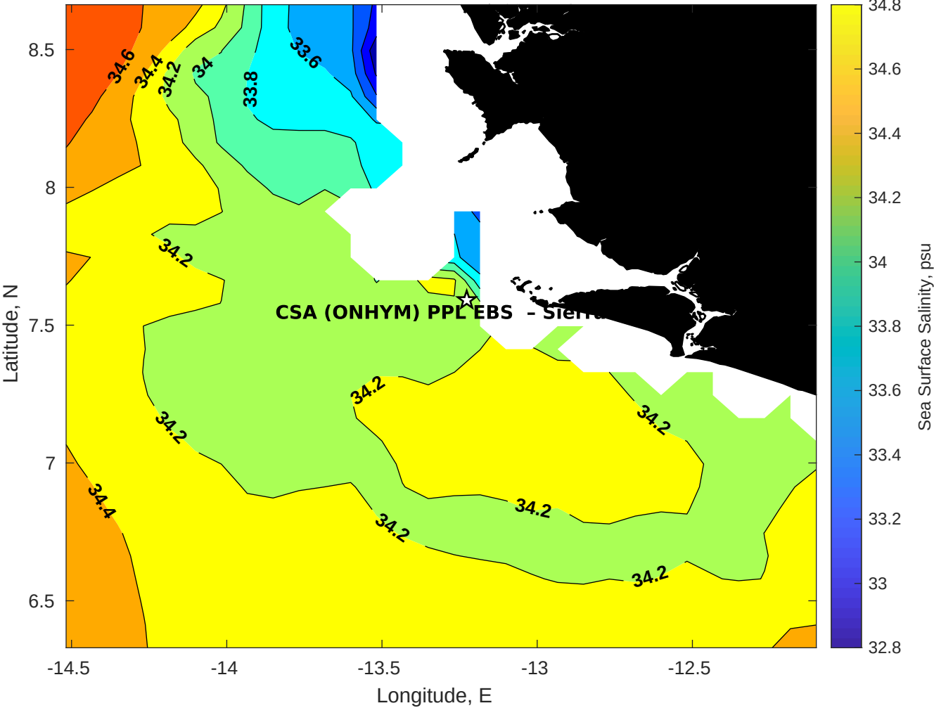
Surface Salinity for CSA (ONHYM) PPL EBS - Sierra Leone at 04-Jan-2026 00:00:00
