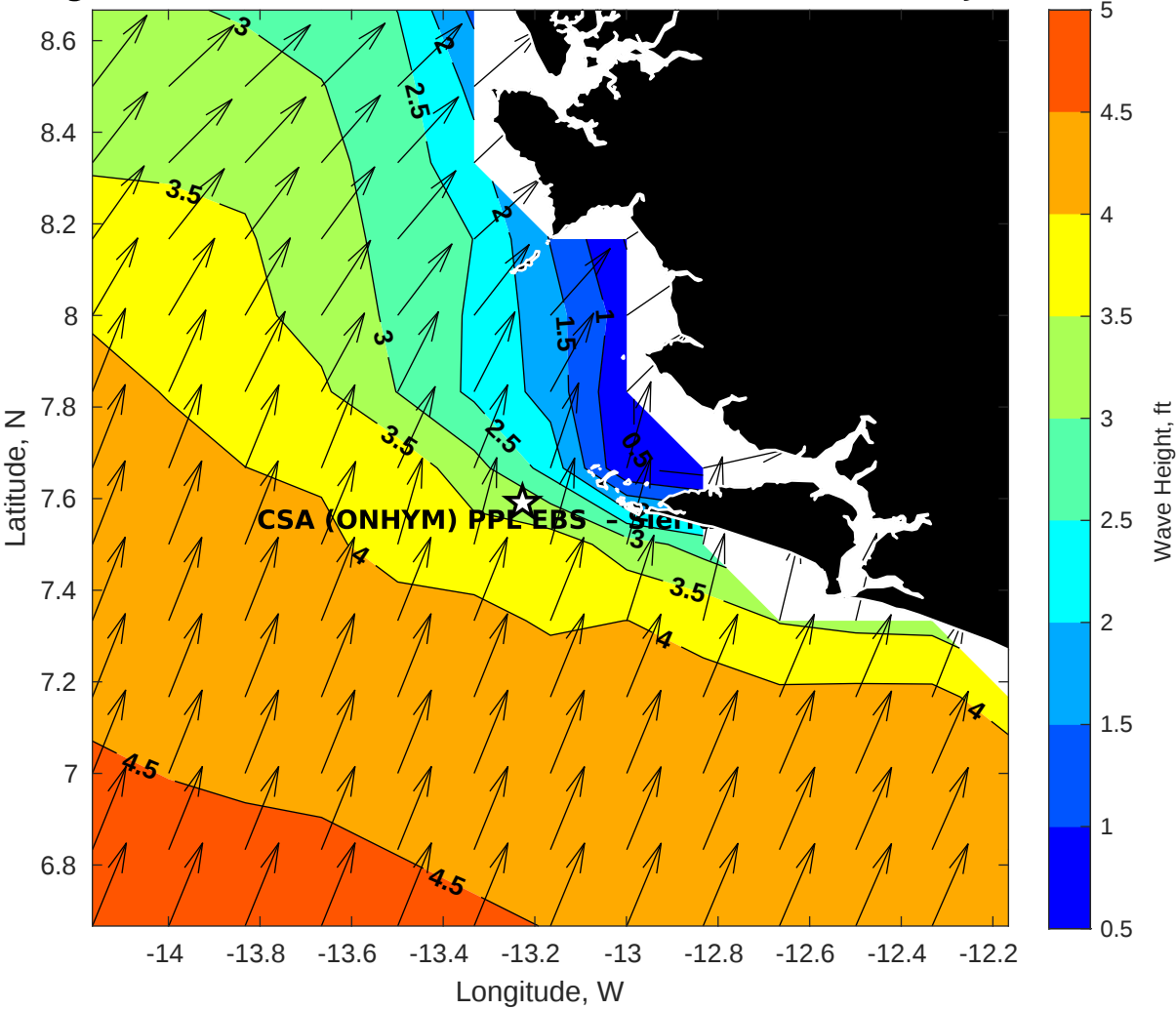
GFS Wave Height (ft) for CSA (ONHYM) PPL EBS - Sierra Leone at 05-Jan-2026 09:00:00
