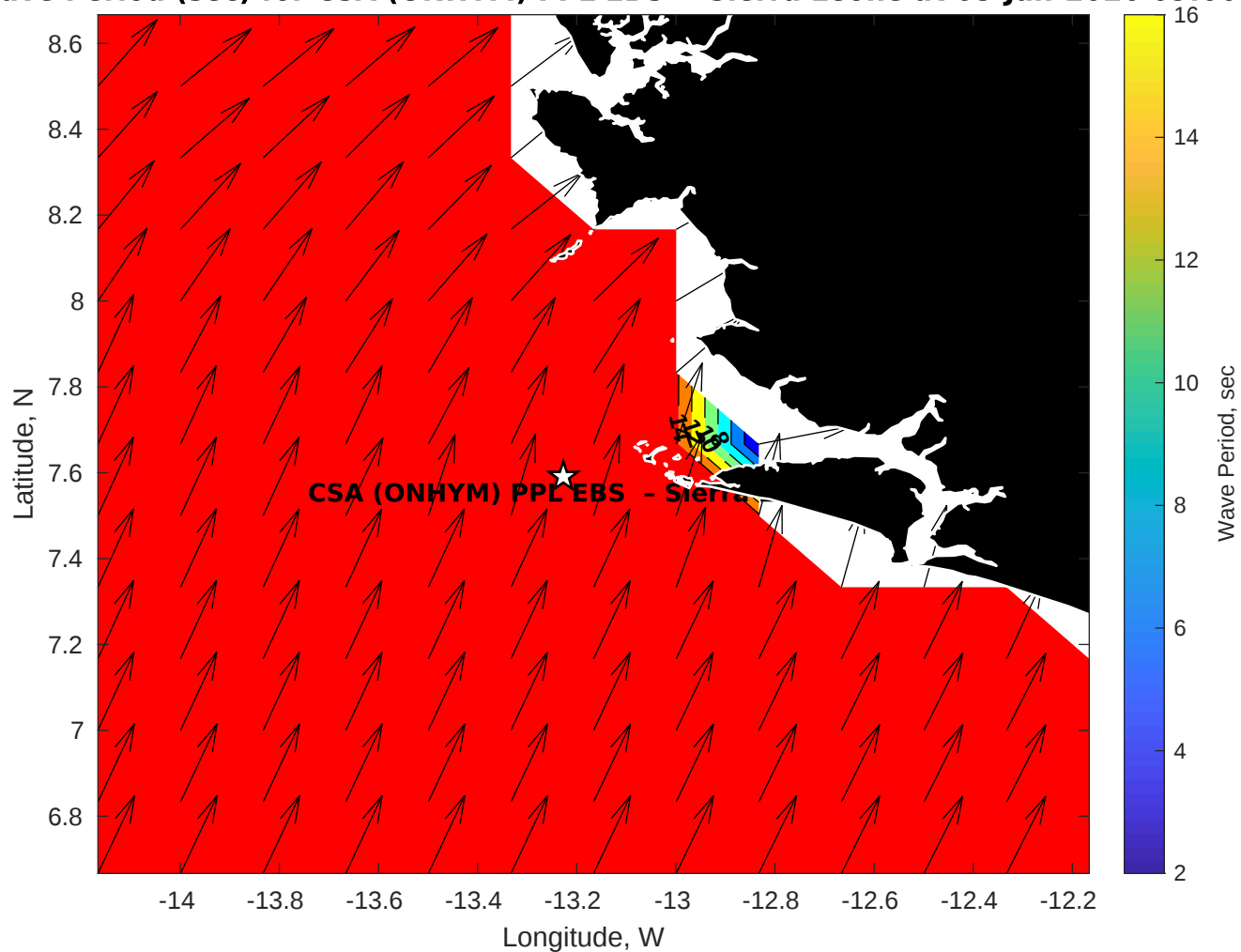
GFS Wave Period (sec) for CSA (ONHYM) PPL EBS - Sierra Leone at 05-Jan-2026 09:00:00
