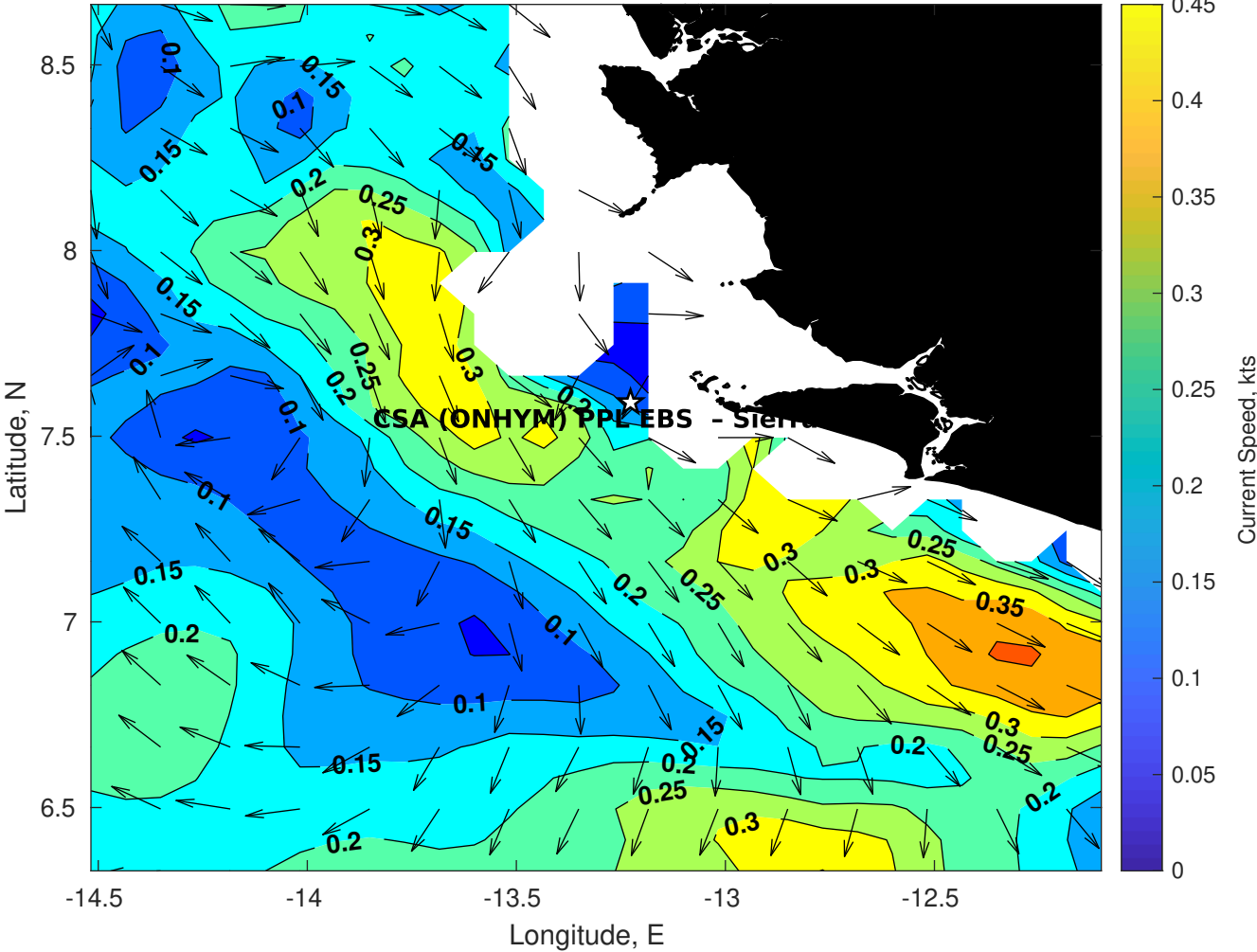
Surface Currents for CSA (ONHYM) PPL EBS - Sierra Leone at 04-Jan-2026 00:00:00
