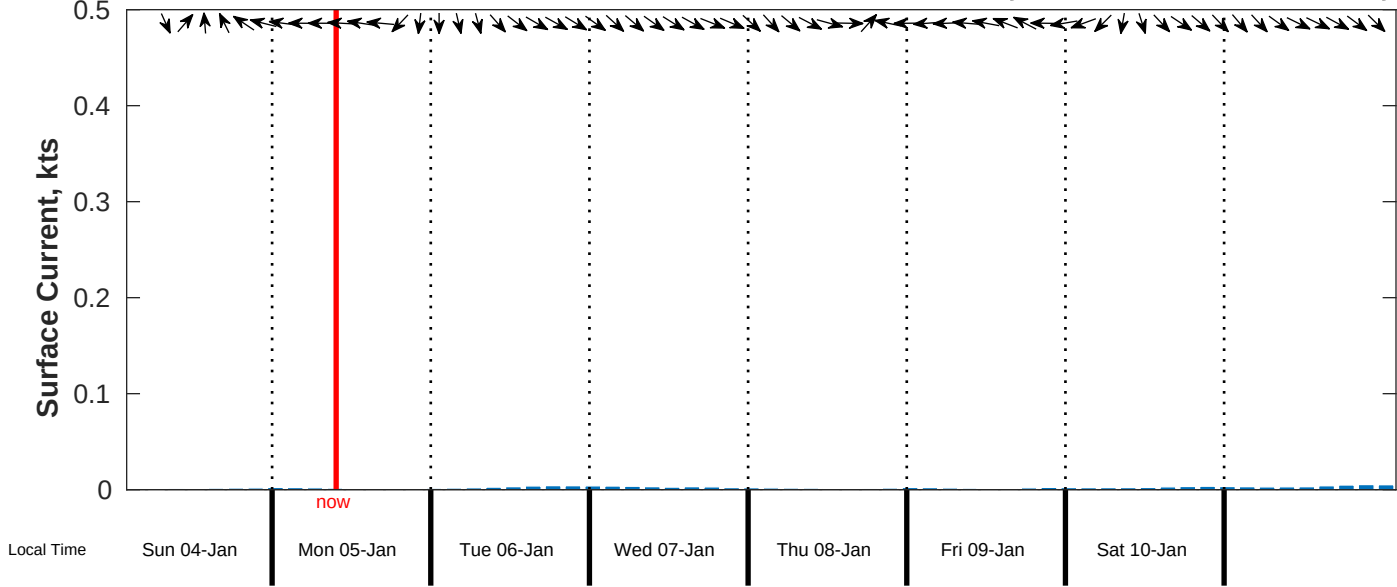
Surface Current Forecast for CSA (ONHYM) PPL EBS - Sierra Leone from 04-Jan-2026 00:00:00 to 12-Jan-2026 00:00:00
