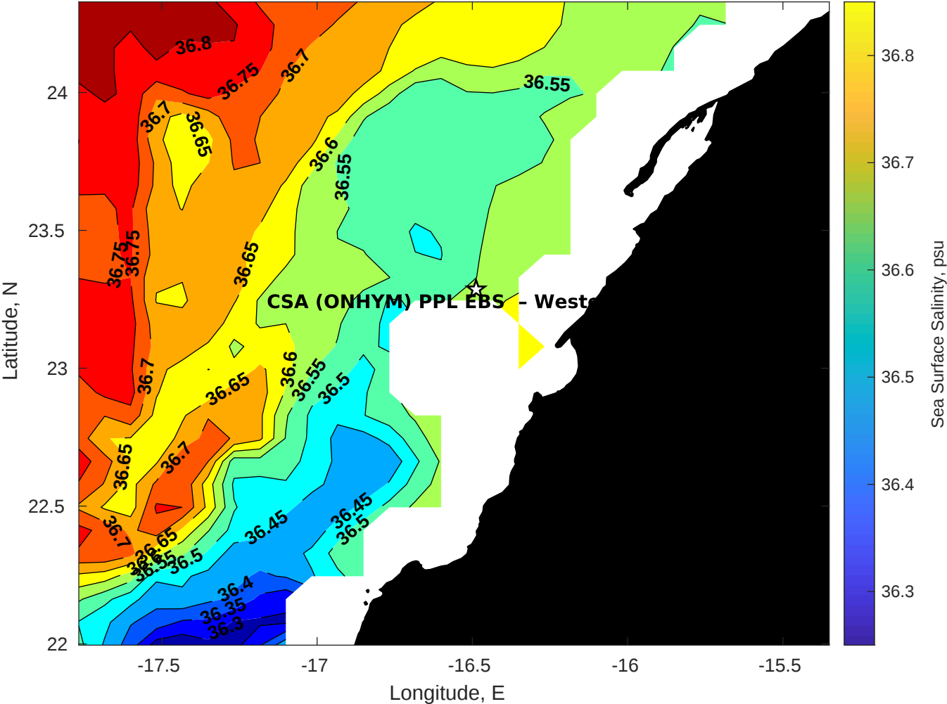
Surface Salinity for CSA (ONHYM) PPL EBS - Western Sahara at 04-Jan-2026 00:00:00
