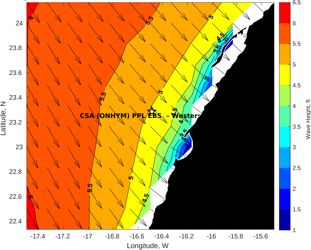
GFS Wave Height (ft) for CSA (ONHYM) PPL EBS - Western Sahara at 05-Jan-2026 09:00:00
