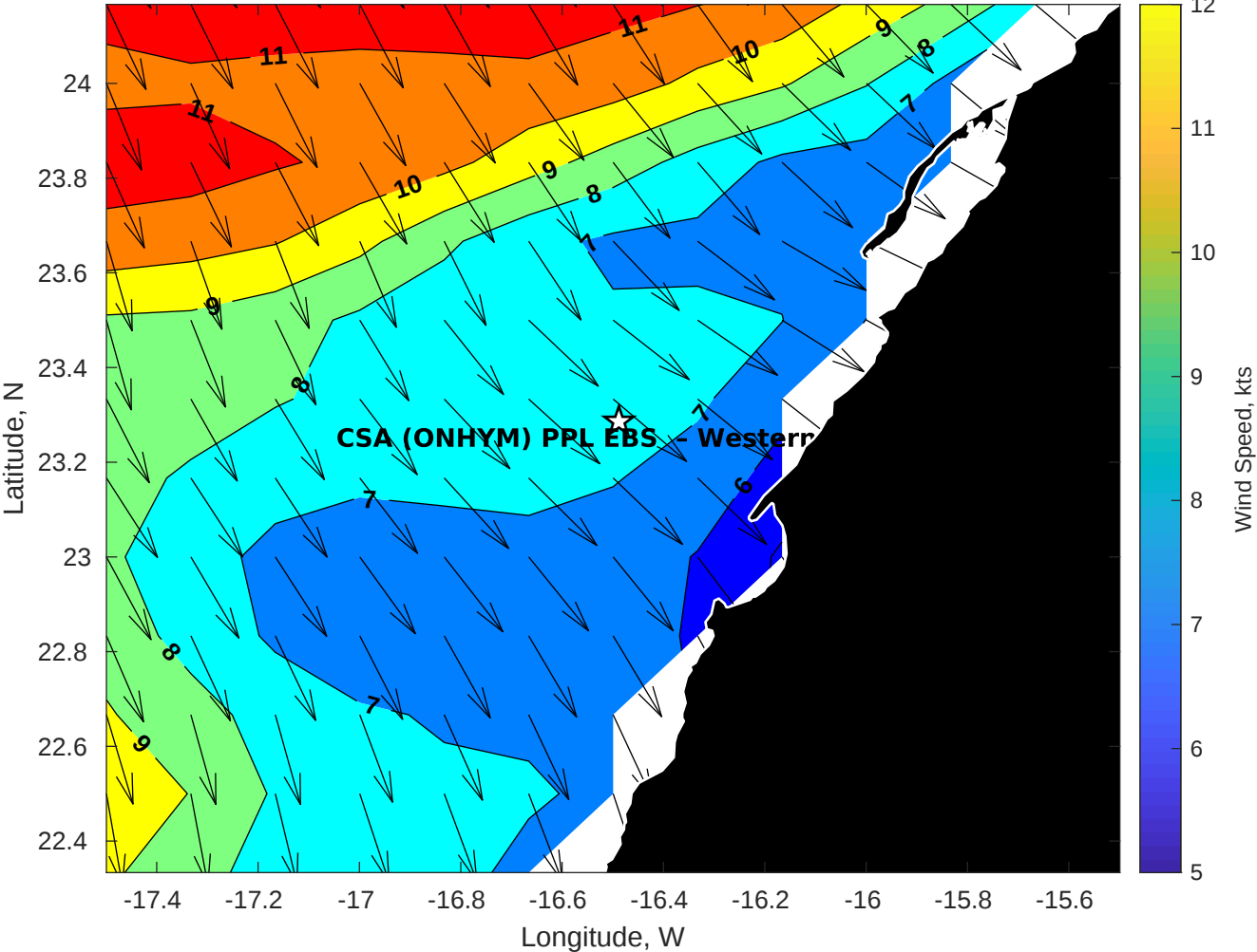
GFS Winds (kts) for CSA (ONHYM) PPL EBS - Western Sahara at 05-Jan-2026 09:00:00
