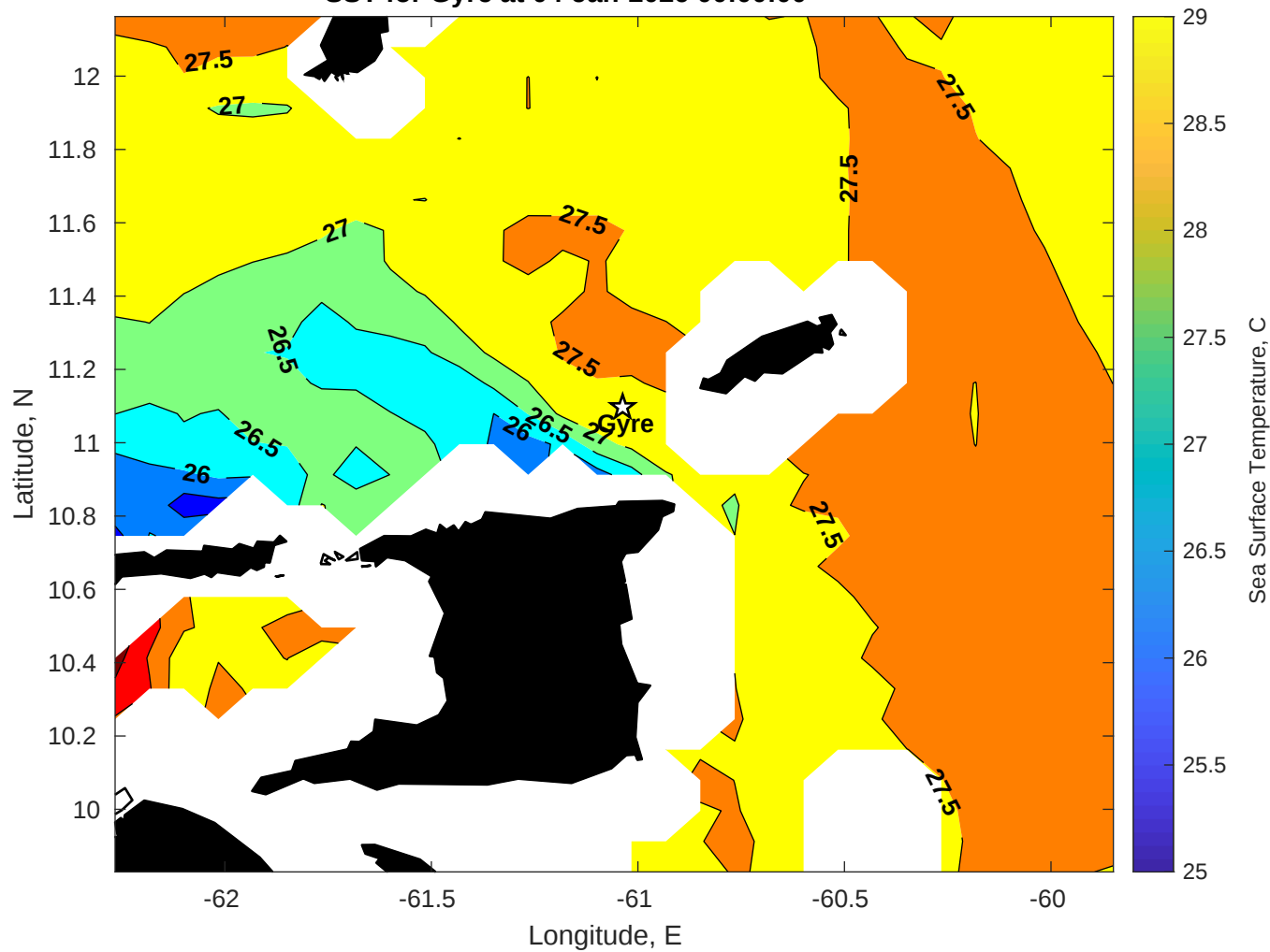
SST for Gyre at 04-Jan-2026 00:00:00
