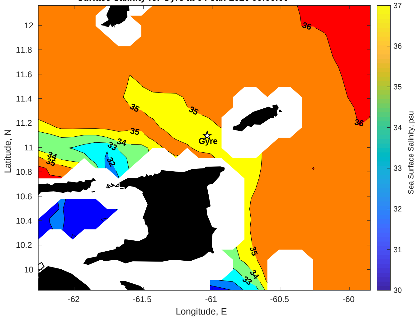
Surface Salinity for Gyre at 04-Jan-2026 00:00:00
