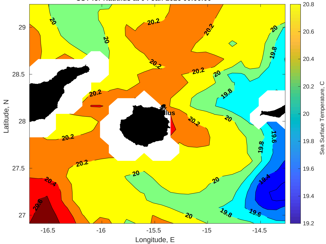
SST for Nautilus at 04-Jan-2026 00:00:00
