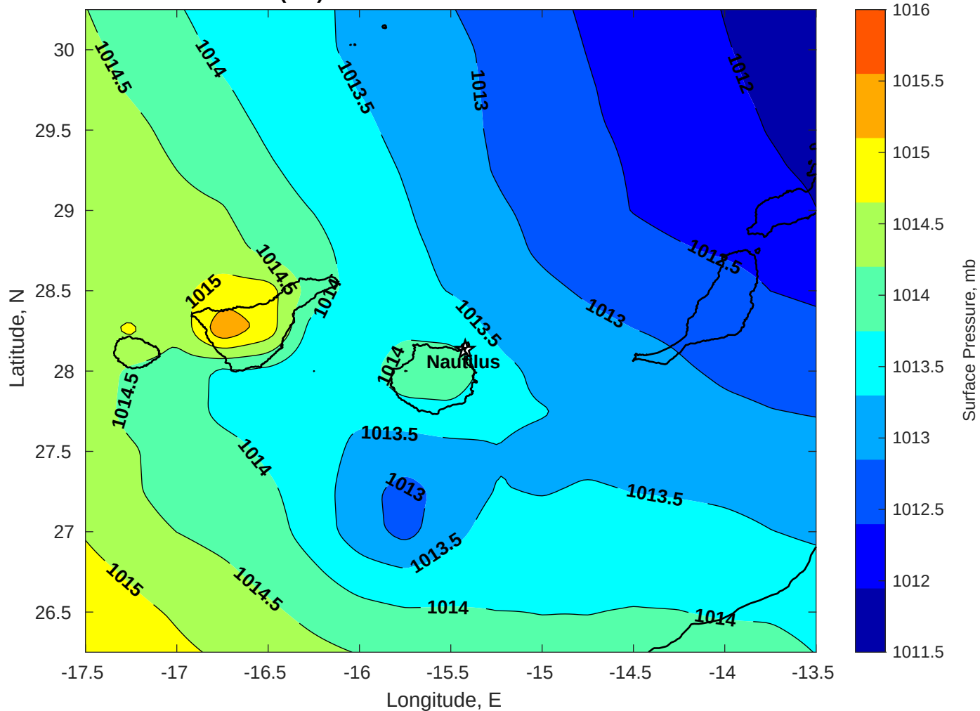
Surface Pressure (mb) for Nautilus at 05-Jan-2026 00:00:00
