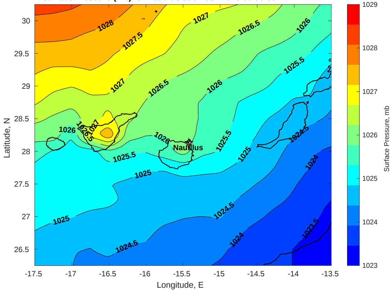
Surface Pressure (mb) for Nautilus at 07-Jan-2026 00:00:00
