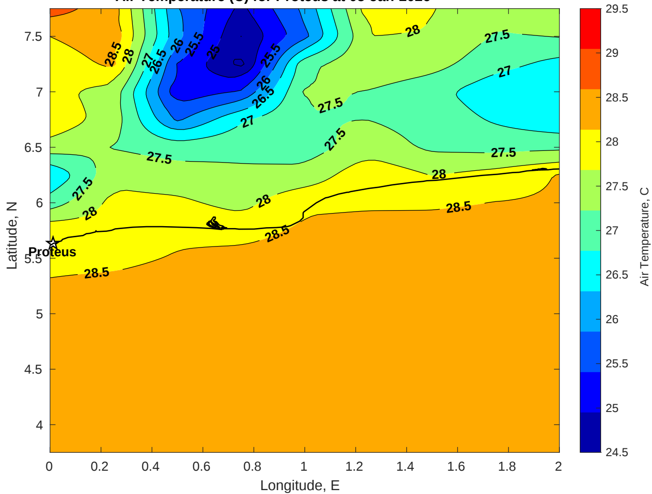
Air Temperature (C) for Proteus at 05-Jan-2026
