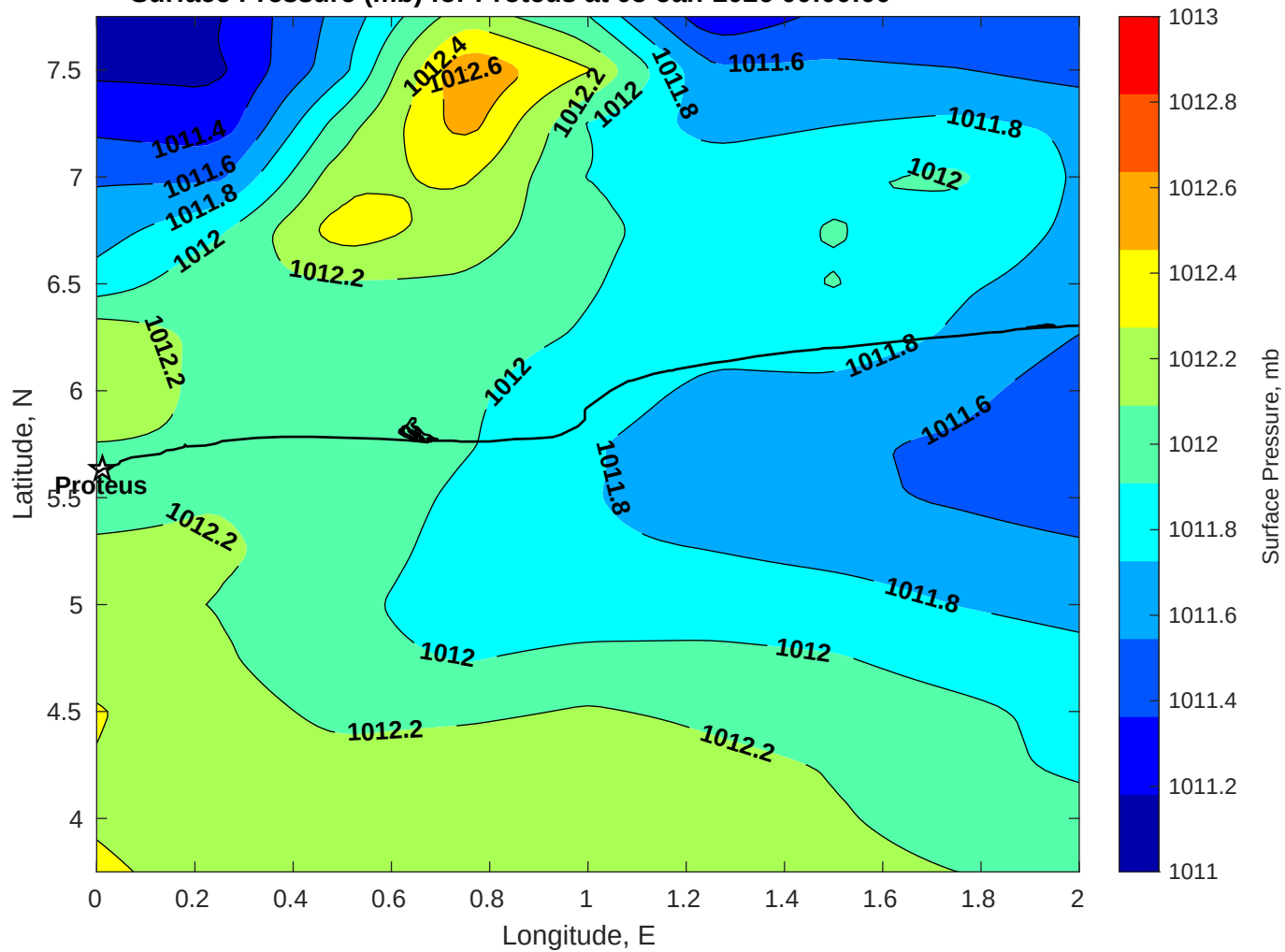
Surface Pressure (mb) for Proteus at 05-Jan-2026 00:00:00
