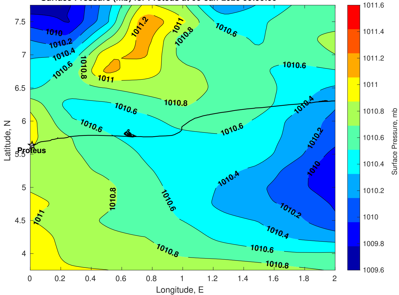
Surface Pressure (mb) for Proteus at 06-Jan-2026 00:00:00
