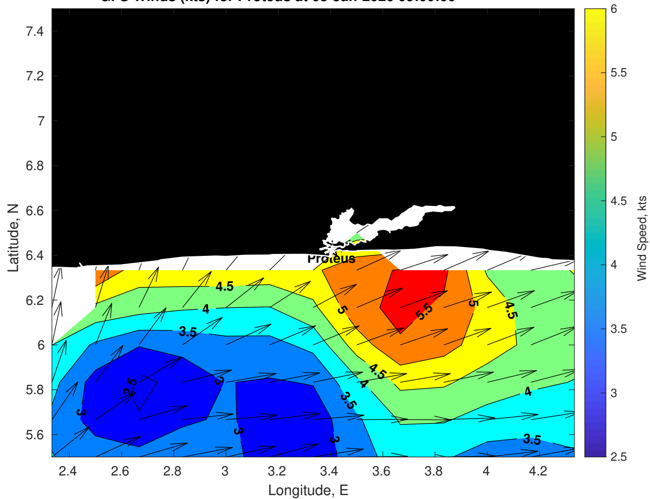
GFS Winds (kts) for Proteus at 03-Jan-2026 09:00:00
