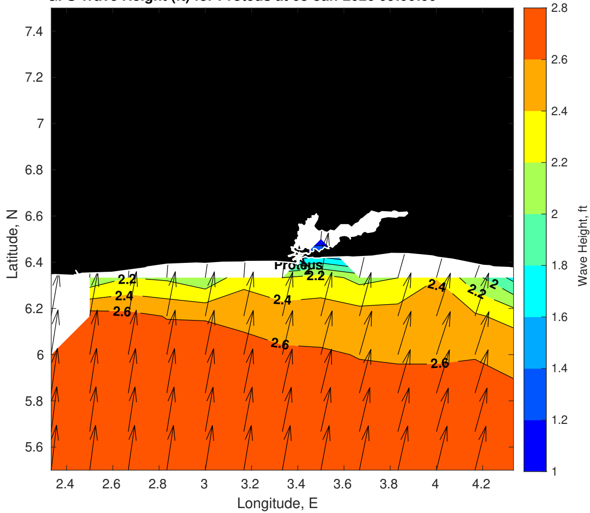
GFS Wave Height (ft) for Proteus at 03-Jan-2026 09:00:00
