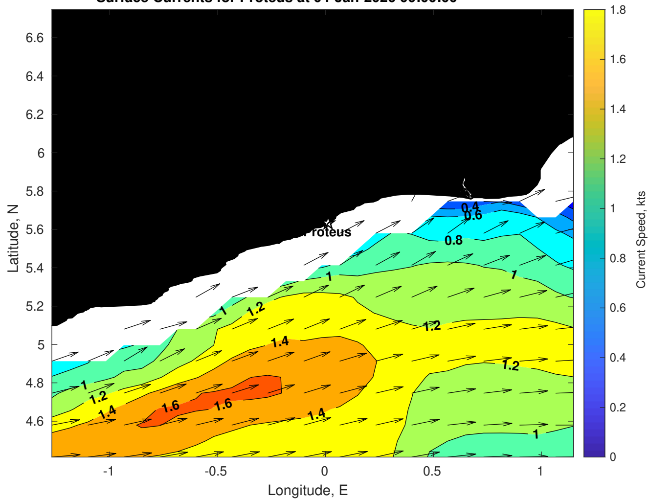
Surface Currents for Proteus at 04-Jan-2026 00:00:00
