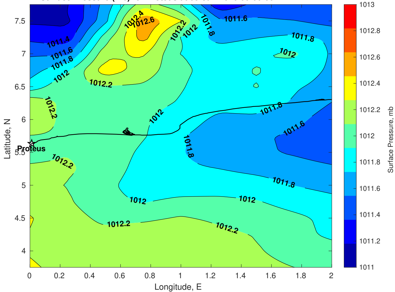
Surface Pressure (mb) for Proteus at 05-Jan-2026 00:00:00
