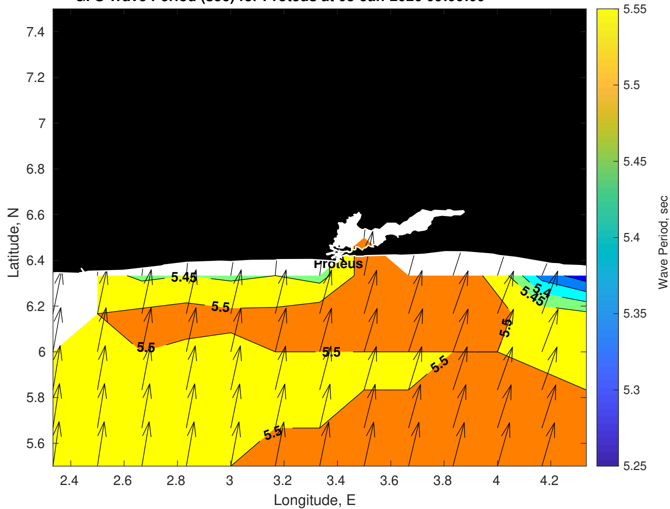
GFS Wave Period (sec) for Proteus at 03-Jan-2026 09:00:00
