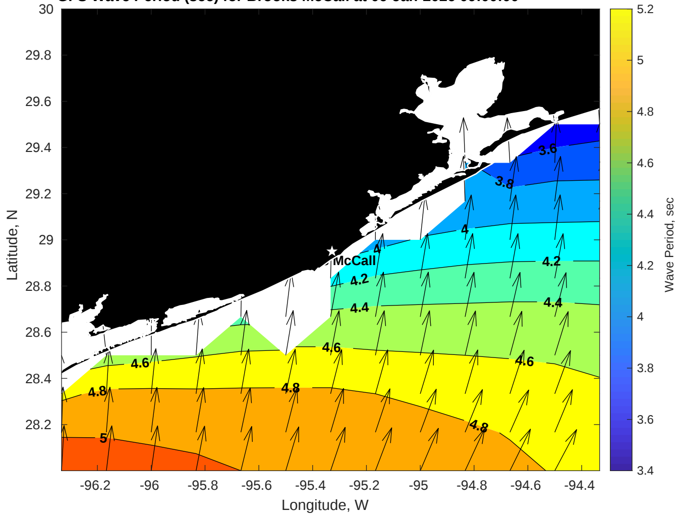
GFS Wave Period (sec) for Brooks McCall at 06-Jan-2026 09:00:00
